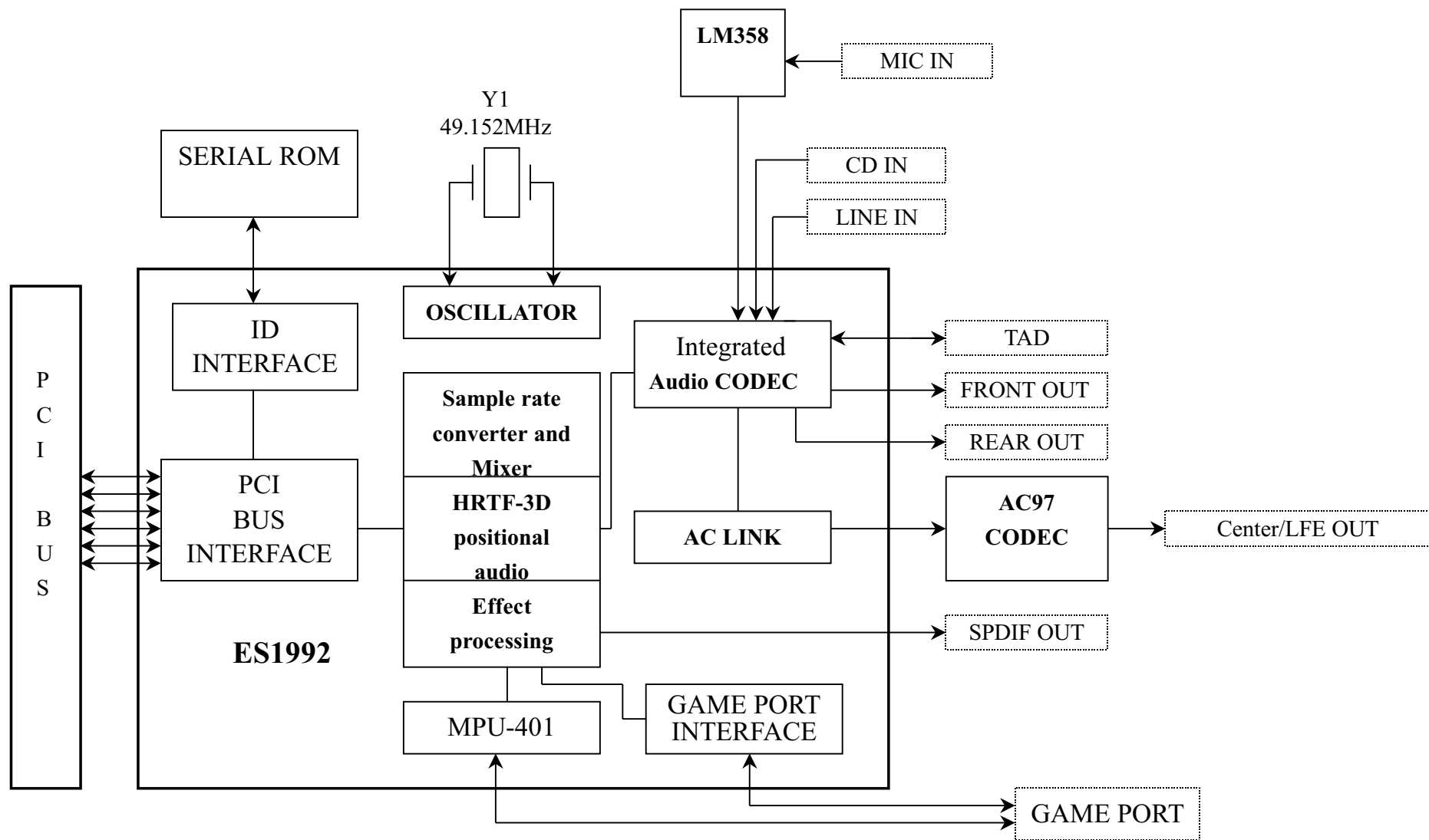
A591-V70 BLOCK DIAGRAM
