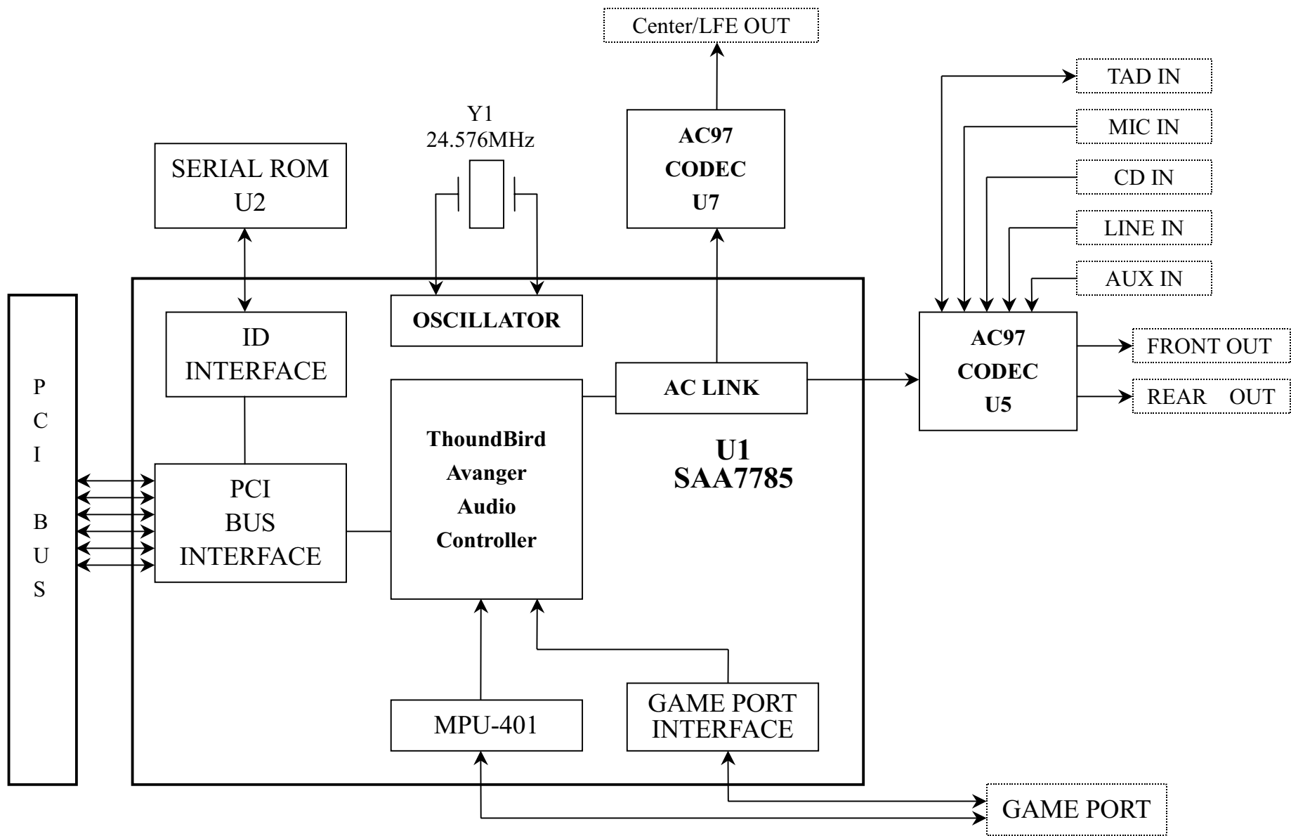
A581-U30 BLOCK DIAGRAM
