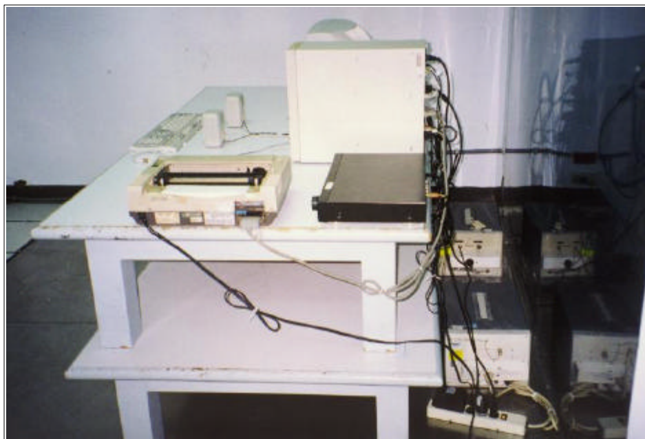
Conducted Emission Setup Photos (Worst Emission Position)
