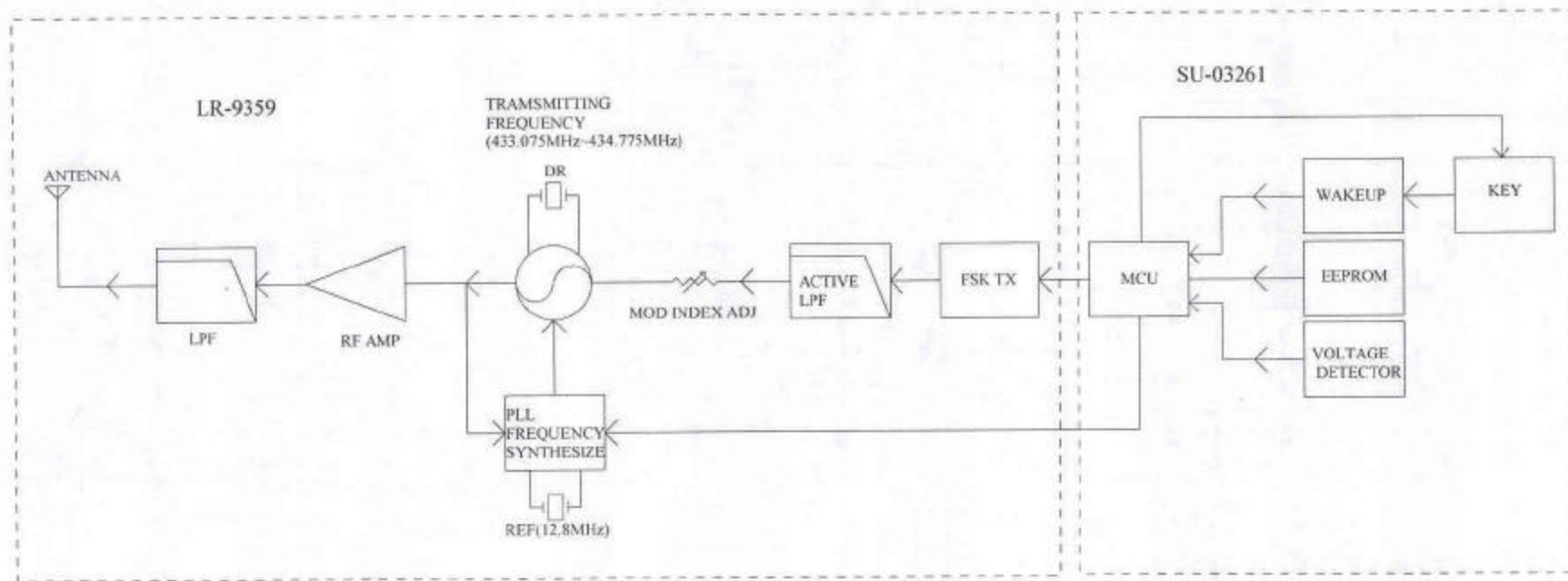
TRANSMITTER FUNCTION BLOCK
