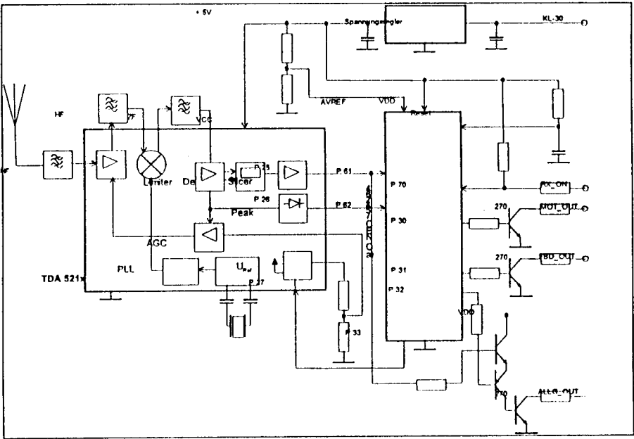
Figure 6: FBD-Receiver internal assembly
