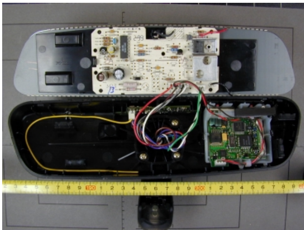
FZV Receiver, FCC ID: LX8FZVE Internal Photographs
