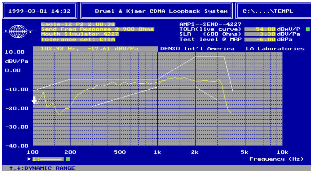
FIGURE 3: Transmit Audio Frequency Response and TOLR (AMPS)
