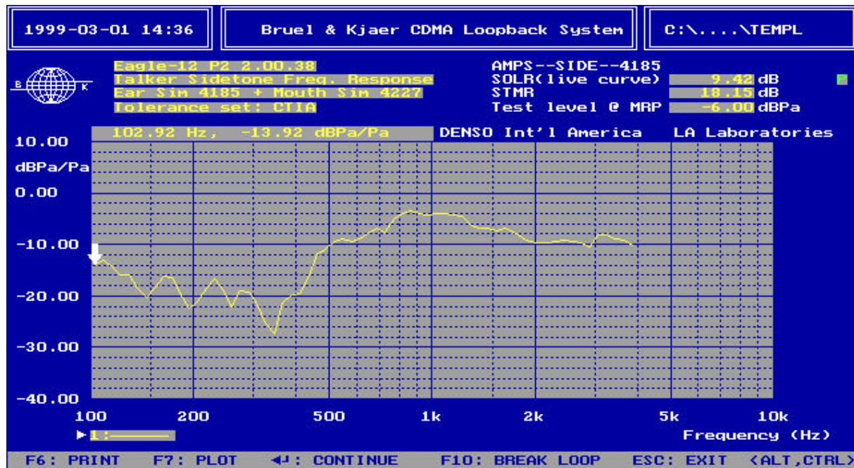
FIGURE 4: Transmit Audio Sidetone Frequency Response and SOLR (AMPS)
