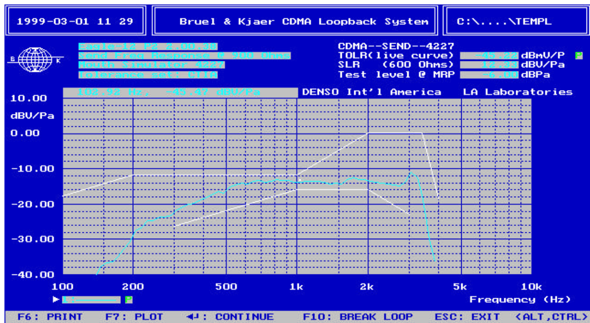
FIGURE 1: Transmit Audio Frequency Response and TOLR (CDMA)
