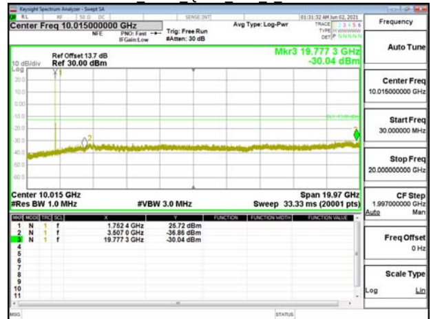
Band4 3MHz QPSK RB1 0 CH20385
