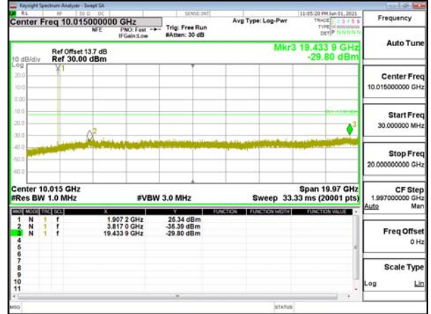
Band2 3MHz QPSK RB1 0 CH19185
