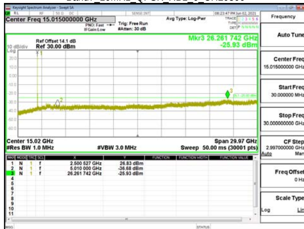
Band7 10MHz QPSK RB1 0 CH21100
