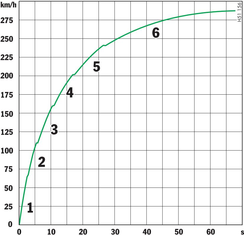
Acceleration diagram for manual transmission – 911 Carrera S
