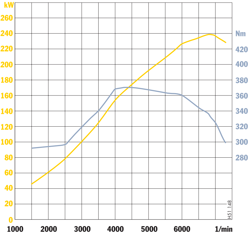
Engine diagram at full power – 911 Carrera
