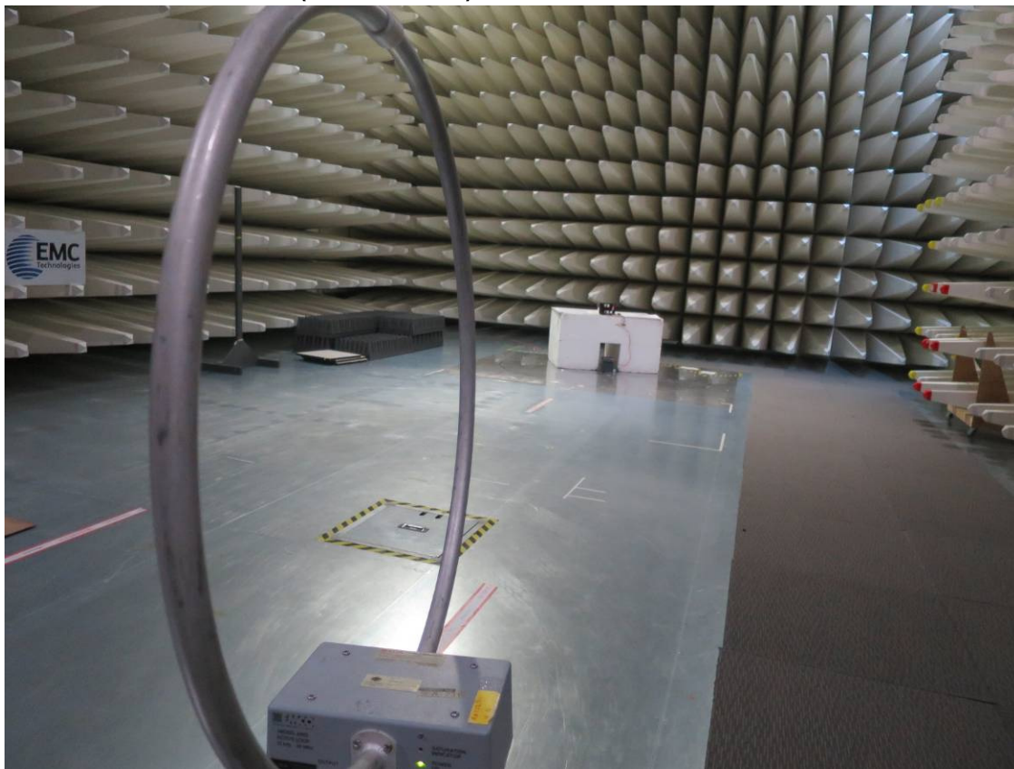
Radiated emissions (below 30 MHz)
