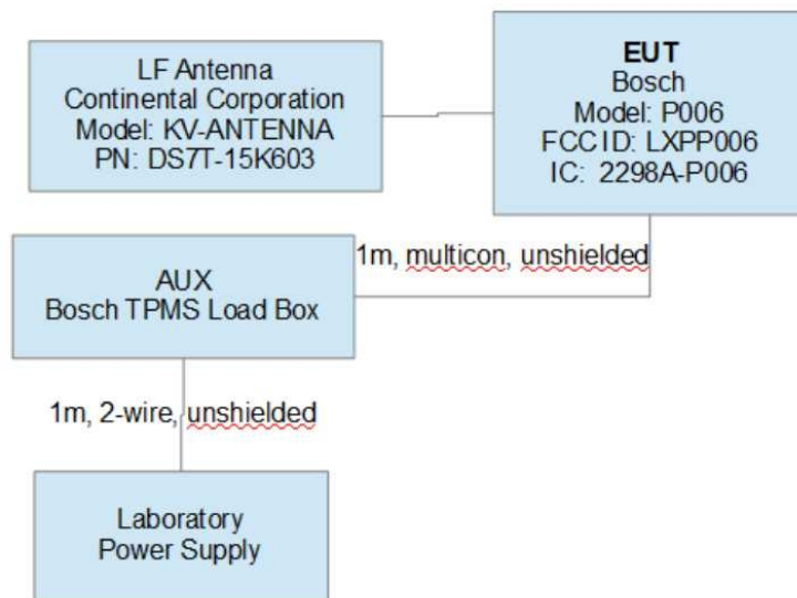
Figure 2: EUT Test Configuration Diagram.
