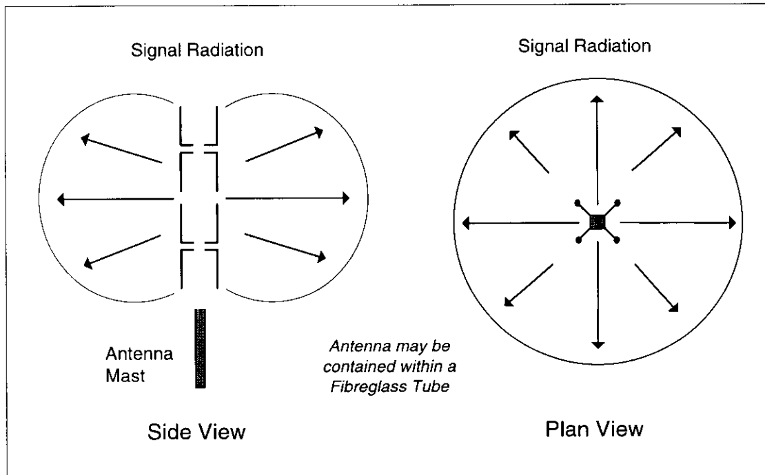
Figure C9. Co-Linear Dipole
