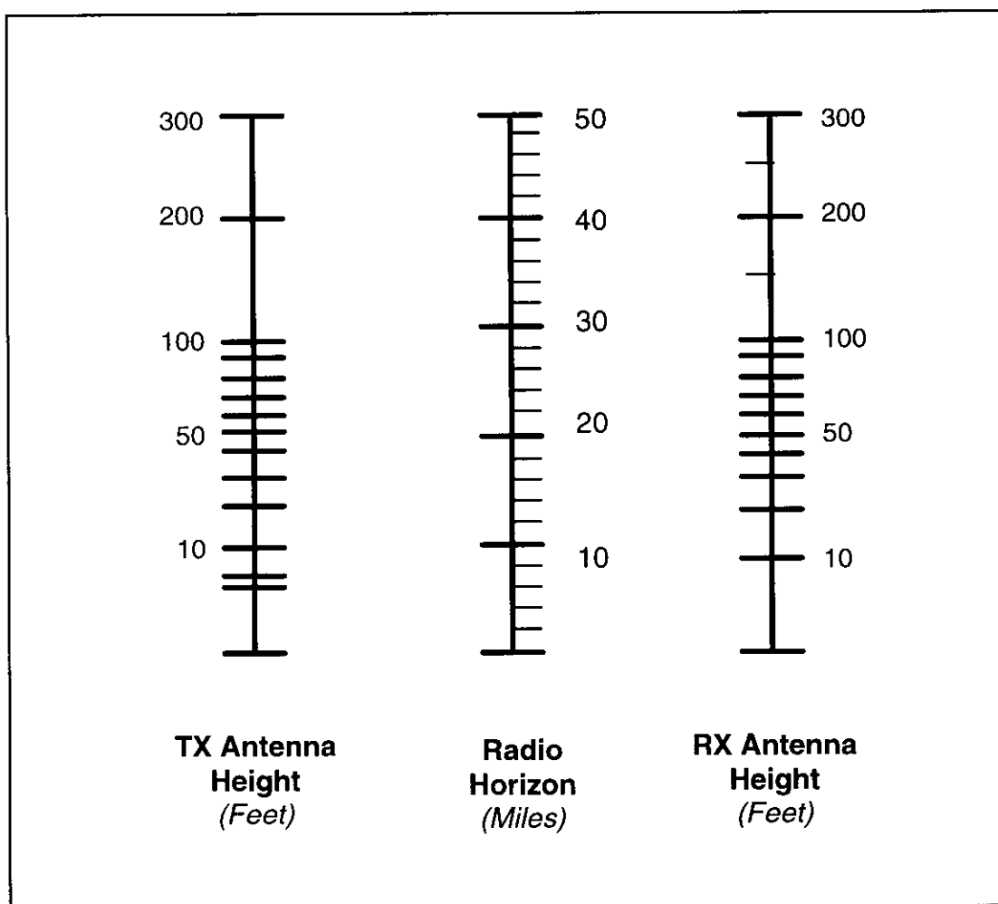
Figure 2.5 Radio Horizon (Feet/Miles)
