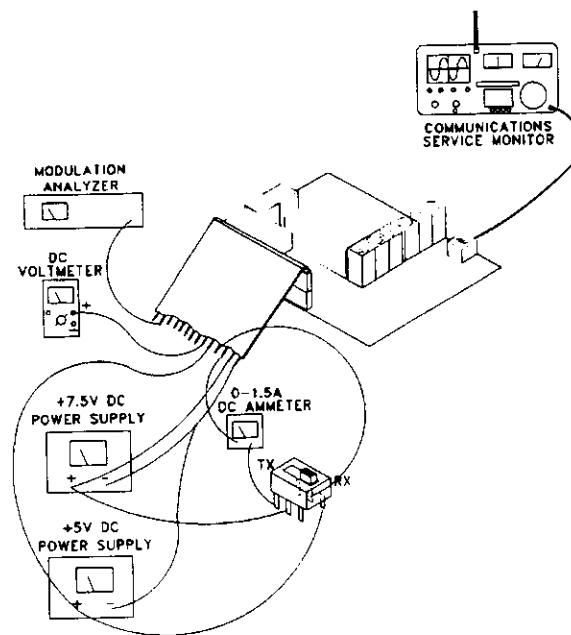
Figure 6-2 RECEIVER TEST SETUP
