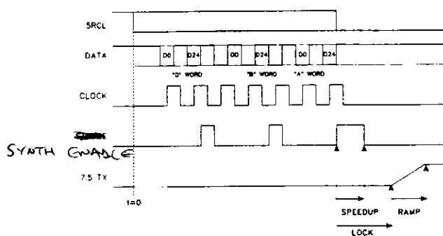
Figure 3-5 RX TO TX TIMING DIAGRAM
