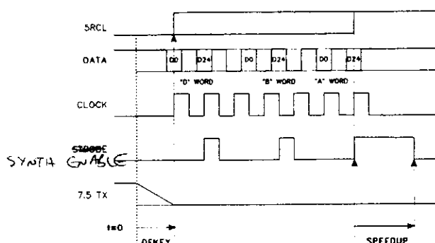
Figure 3-6 TX TO RX TIMING DIAGRAM
