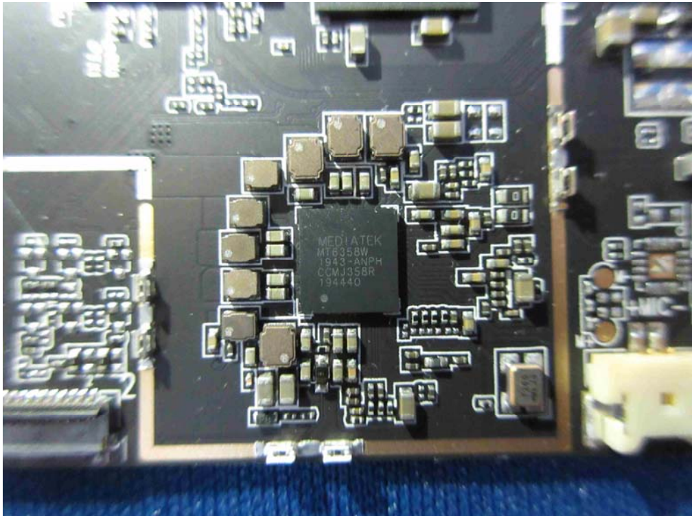
(25) EUT Photo
