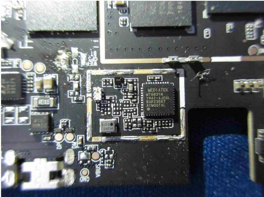
(28) EUT Photo
