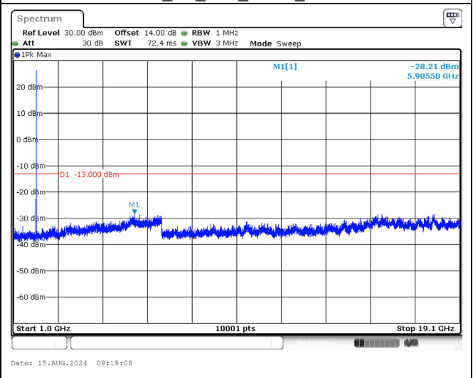
1908.5 MHz_3M_1RB_QPSK_Above 1GHz
