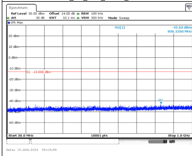
1908.5 MHz_3M_1RB_QPSK_Below 1GHz
