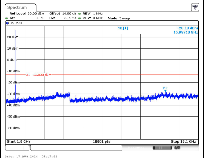
1908.5 MHz_3M_1RB_QPSK_Above 1GHz
