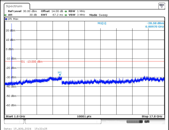
LTE Band 66_1745.0 MHz_10M_1RB_QPSK_Above 1GHz
