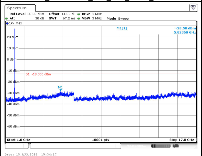
1775.0MHz_10M_1RB_QPSK_Above 1GHz
