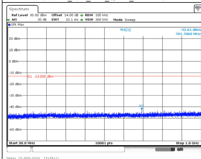
1775.0MHz_10M_1RB_QPSK_Below 1GHz
