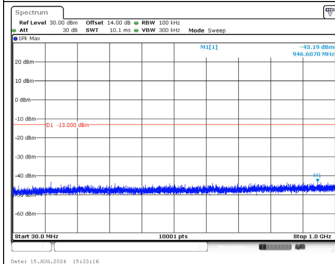
LTE Band 66_1745.0 MHz_10M_1RB_QPSK_Below 1GHz
