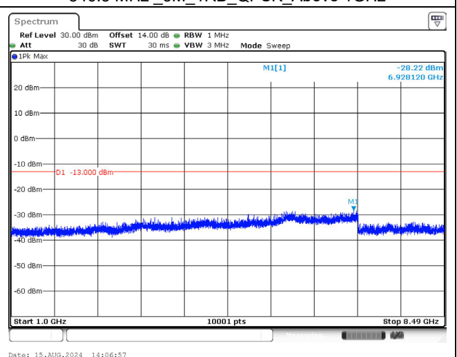
846.5 MHz_5M_1RB_QPSK_Above 1GHz
