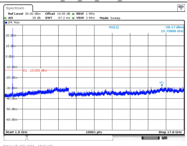
1770.0 MHz_20M_1RB_QPSK_Above 1GHz
