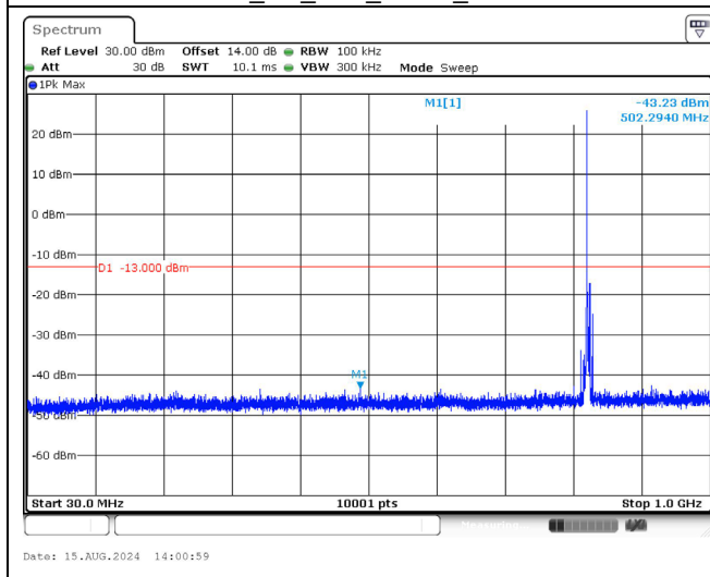
836.5 MHz_5M_1RB_QPSK_Below 1GHz
