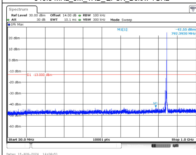
846.5 MHz_5M_1RB_QPSK_Below 1GHz
