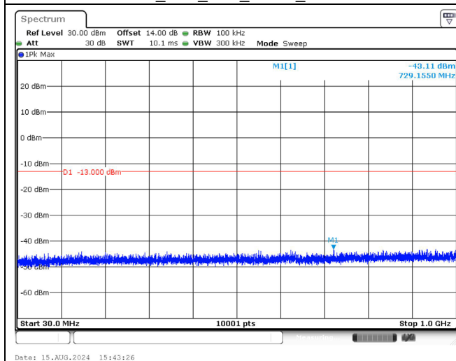
1745.0 MHz_15M_1RB_QPSK_Below 1GHz
