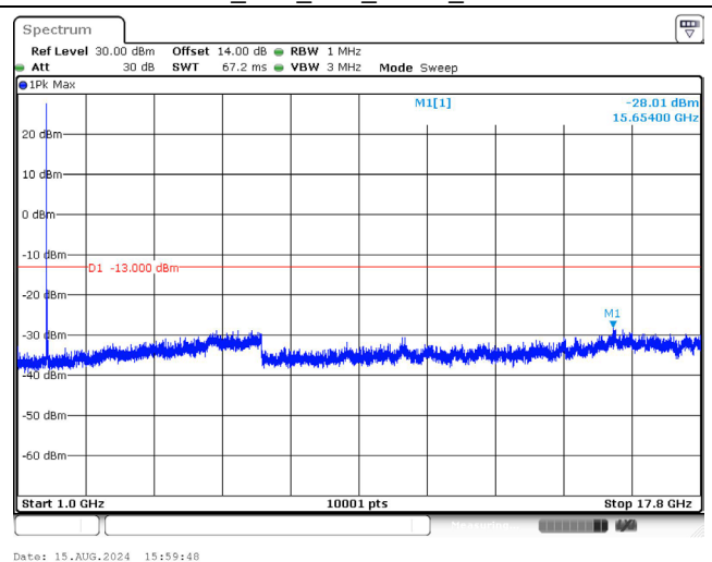
1745.0 MHz_20M_1RB_QPSK_Above 1GHz
