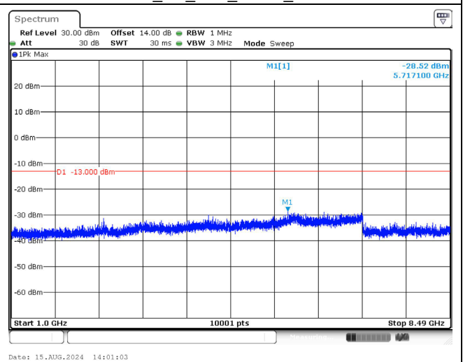
836.5 MHz_5M_1RB_QPSK_Above 1GHz
