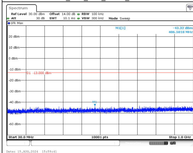
1745.0 MHz_20M_1RB_QPSK_Below 1GHz
