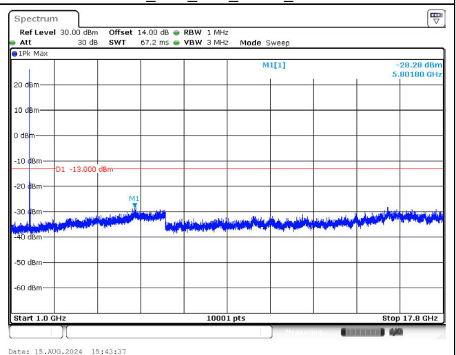
1745.0 MHz_15M_1RB_QPSK_Above 1GHz
