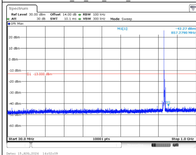
846.5 MHz_5M_1RB_QPSK_Below 1GHz
