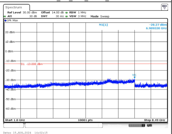
846.5 MHz_5M_1RB_QPSK_Above 1GHz
