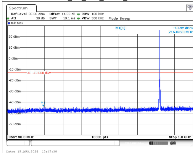
836.5 MHz_3M_1RB_QPSK_Below 1GHz
