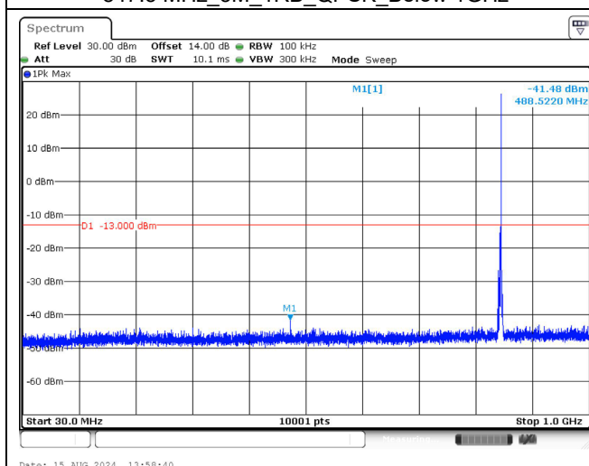
847.5 MHz_3M_1RB_QPSK_Below 1GHz
