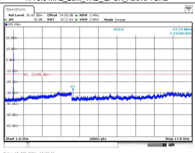
1770.0 MHz_20M_1RB_QPSK_Above 1GHz
