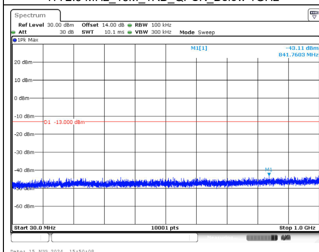
1772.5 MHz_15M_1RB_QPSK_Below 1GHz
