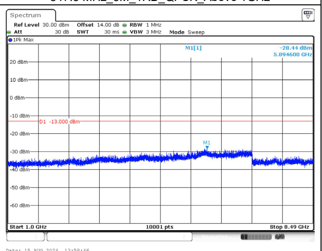
847.5 MHz_3M_1RB_QPSK_Above 1GHz
