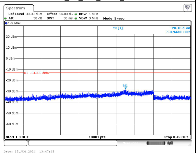
836.5 MHz_3M_1RB_QPSK_Above 1GHz
