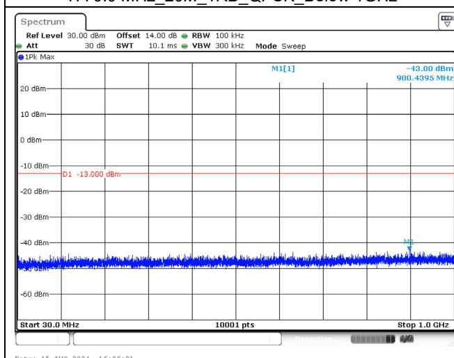
1770.0 MHz_20M_1RB_QPSK_Below 1GHz
