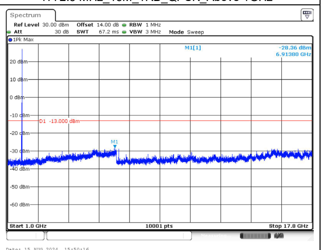
1772.5 MHz_15M_1RB_QPSK_Above 1GHz
