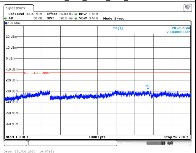
2535.0 MHz_10M_QPSK_1RB_Above 1GHz
