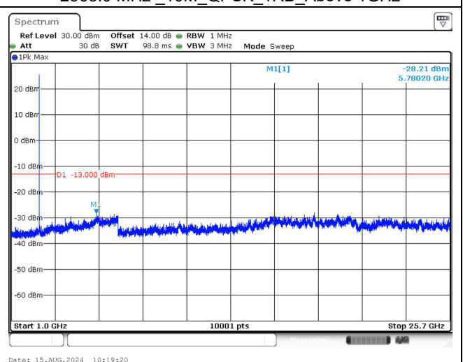
2565.0 MHz_10M_QPSK_1RB_Above 1GHz
