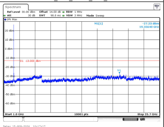
2565.0 MHz_10M_QPSK_1RB_Above 1GHz
