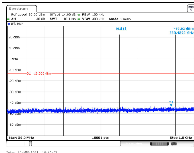
2560.0 MHz _20M_QPSK_1RB_Below 1GHz
