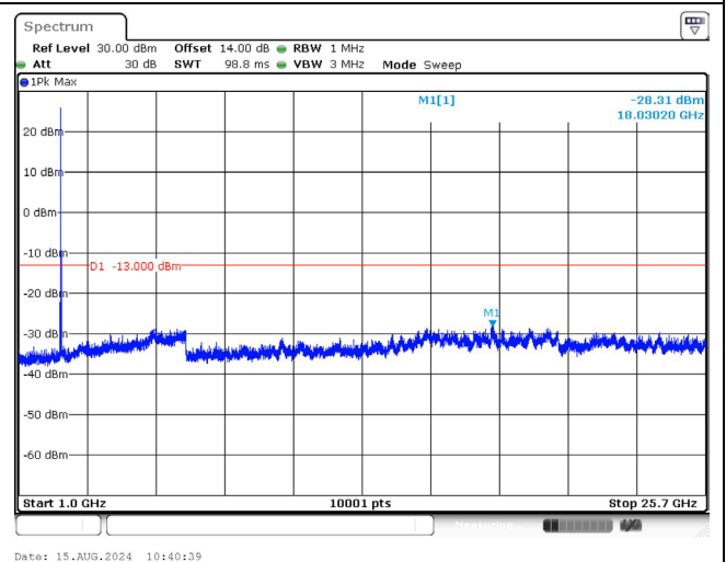
2535.0 MHz _20M_QPSK_1RB_Above 1GHz
