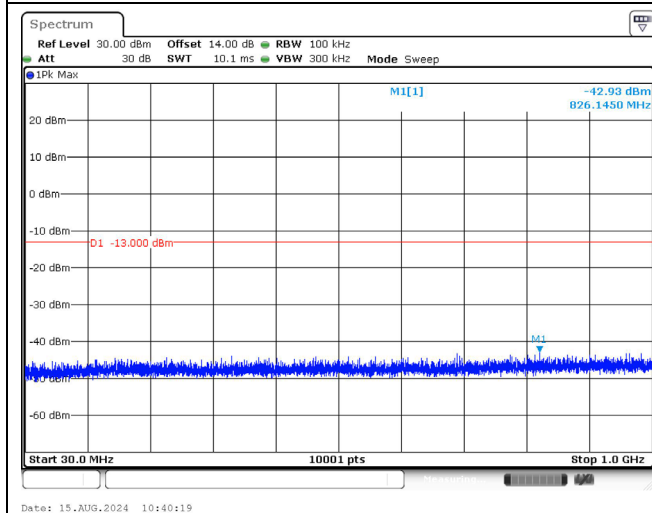
2535.0 MHz _20M_QPSK_1RB_Below 1GHz
