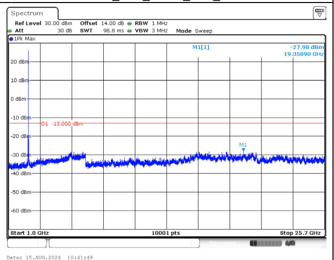
2560.0 MHz _20M_QPSK_1RB_Above 1GHz
