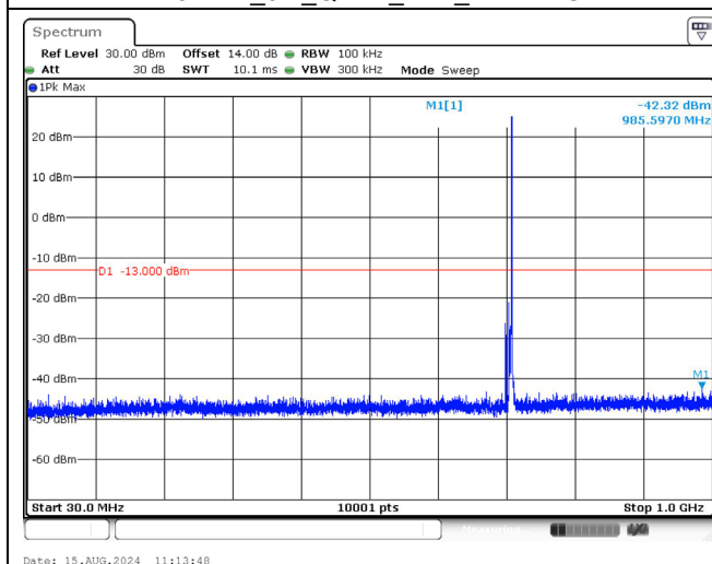
714.5 MHz_5M_QPSK_1RB_Below 1GHz
