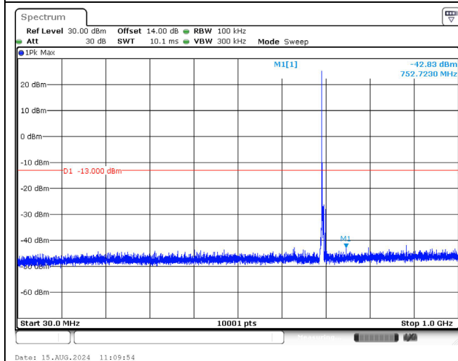
707.5 MHz_5M_QPSK_1RB_Below 1GHz
