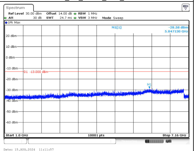
714.5 MHz_5M_QPSK_1RB_Above 1GHz
