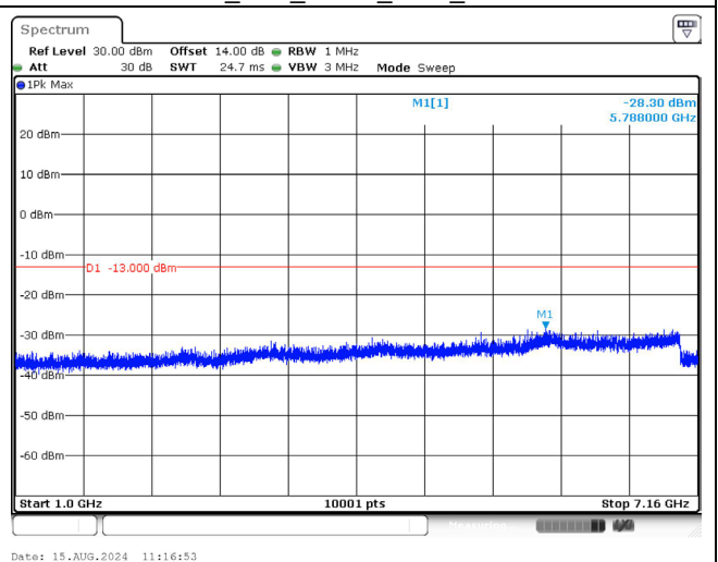
707.5 MHz_10M_QPSK_1RB_Above 1GHz
