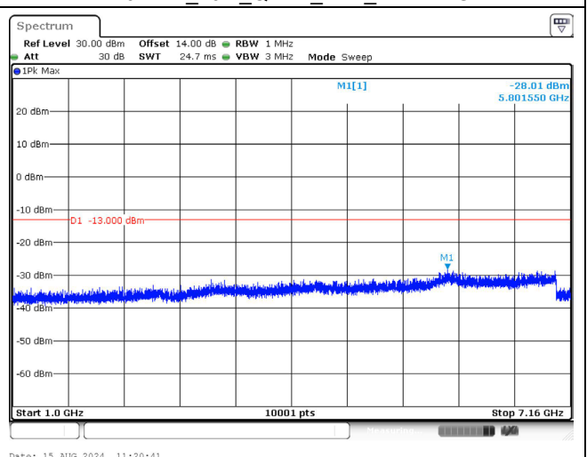
711.0 MHz_10M_QPSK_1RB_Above 1GHz
