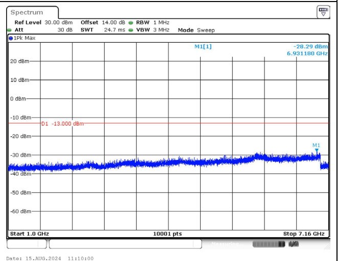
707.5 MHz_5M_QPSK_1RB_Above 1GHz
