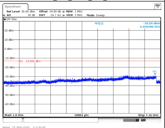
711.0 MHz_10M_QPSK_1RB_Above 1GHz
