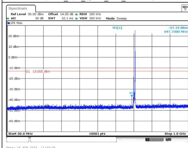
711.0 MHz_10M_QPSK_1RB_Below 1GHz
