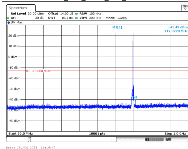
707.5 MHz_10M_QPSK_1RB_Below 1GHz
