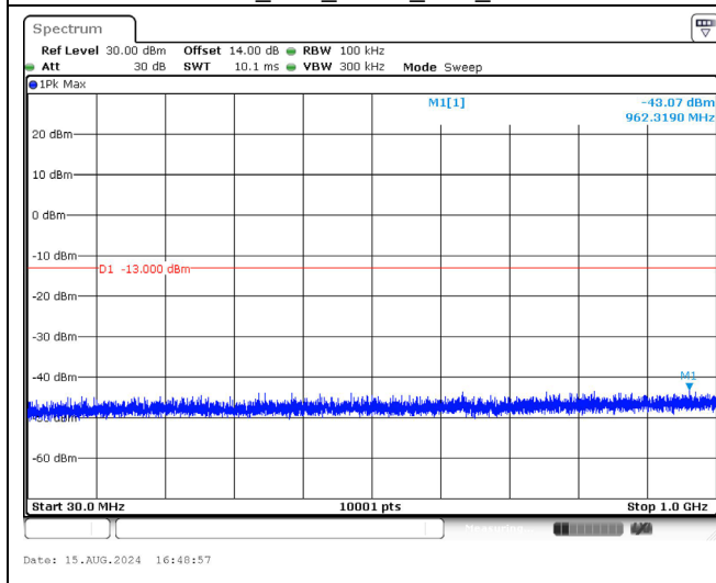
2615.0 MHz_10M_QPSK_1RB_Below 1GHz
