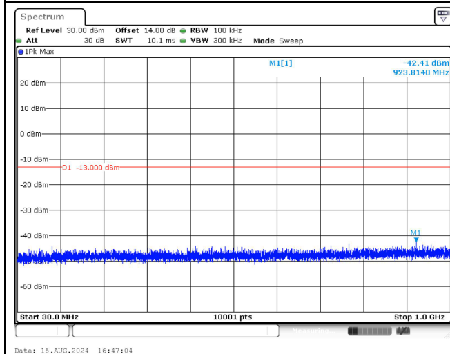
2615.0 MHz_10M_QPSK_1RB_Below 1GHz
