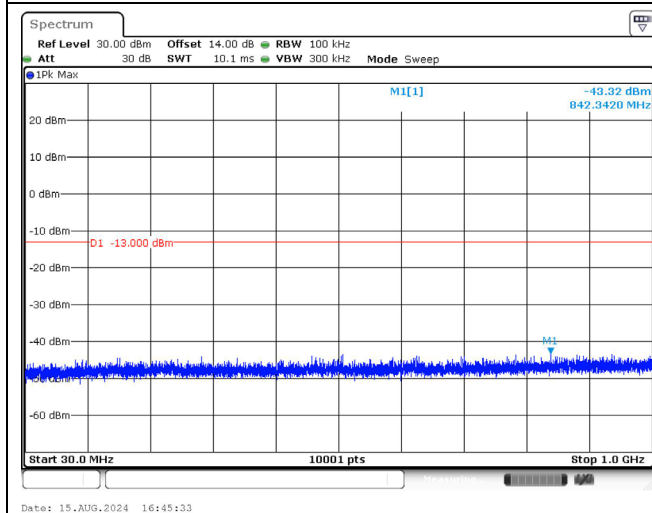
2595.0 MHz_10M_QPSK_1RB_Below 1GHz
