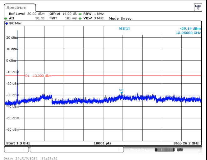
2595.0 MHz_10M_QPSK_1RB_Above 1GHz
