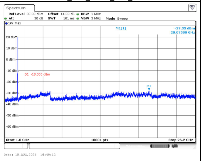
2615.0 MHz_10M_QPSK_1RB_Above 1GHz
