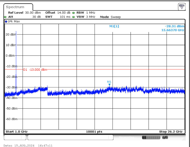
2615.0 MHz_10M_QPSK_1RB_Above 1GHz
