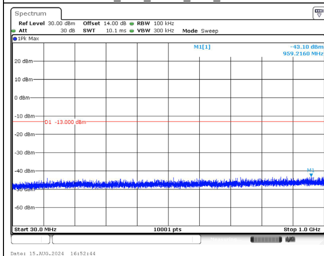
2595.0 MHz_15M_QPSK_1RB_Below 1GHz
