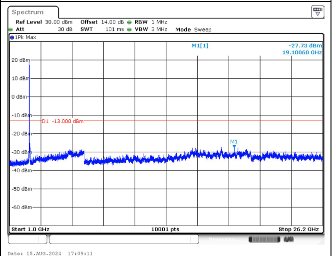
2595.0 MHz _20M_QPSK_1RB_Above 1GHz
