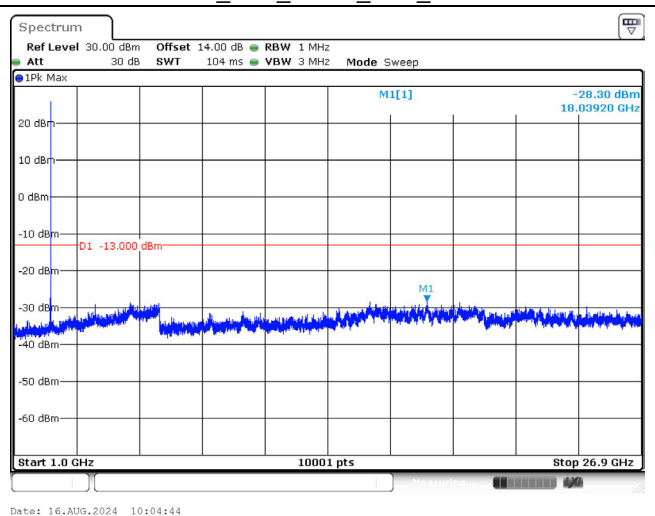
2593.0 MHz_10M_QPSK_1RB_Above 1GHz
