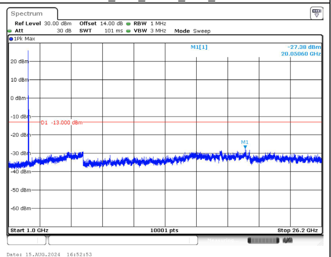
2595.0 MHz_15M_QPSK_1RB_Above 1GHz
