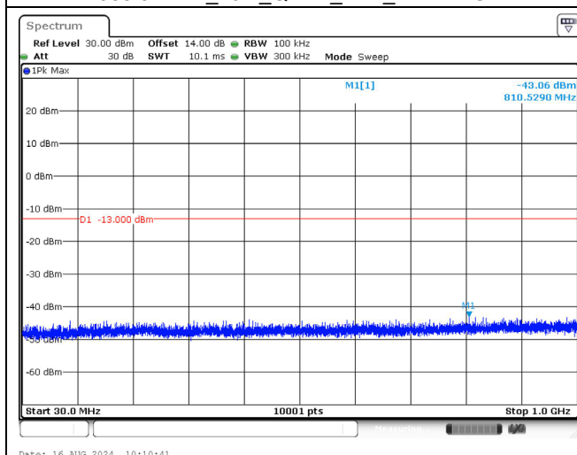
2685.0 MHz_10M_QPSK_1RB_Below 1GHz
