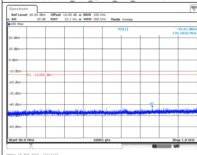
2610.0 MHz _20M_QPSK_1RB_Below 1GHz
