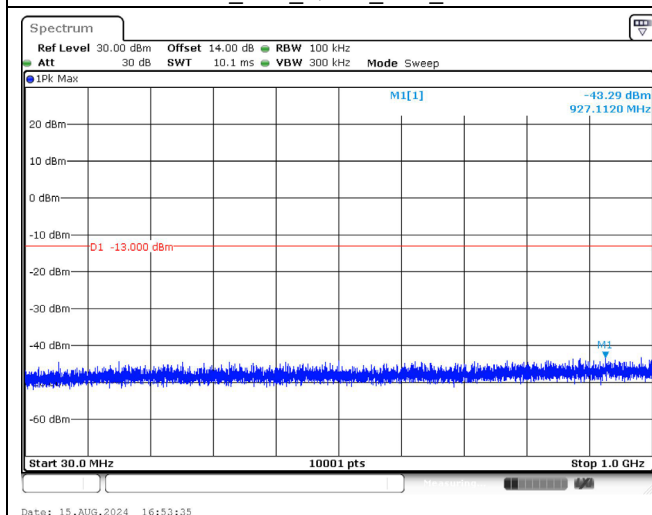
2612.5 MHz_15M_QPSK_1RB_Below 1GHz
