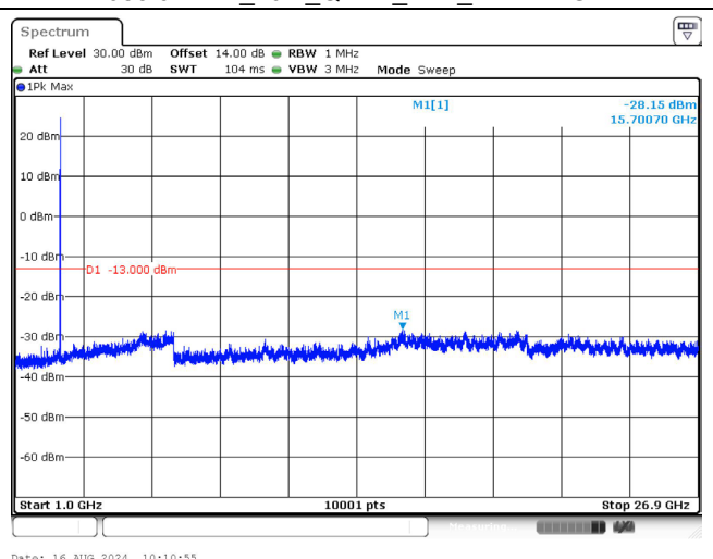
2685.0 MHz_10M_QPSK_1RB_Above 1GHz
