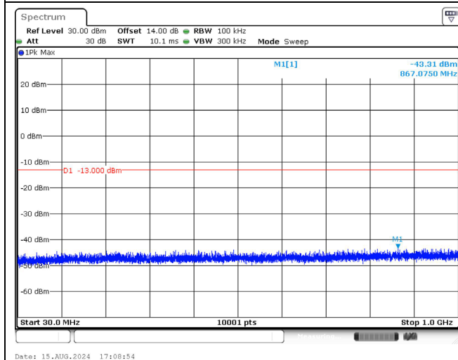
2595.0 MHz _20M_QPSK_1RB_Below 1GHz
