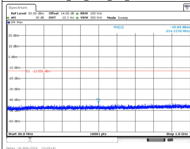
2685.0 MHz_10M_QPSK_1RB_Below 1GHz
