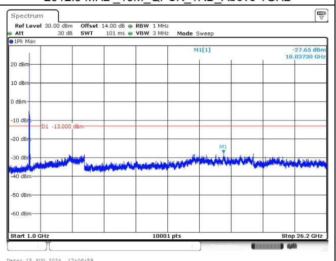
2612.5 MHz_15M_QPSK_1RB_Above 1GHz
