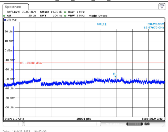
2685.0 MHz_10M_QPSK_1RB_Above 1GHz
