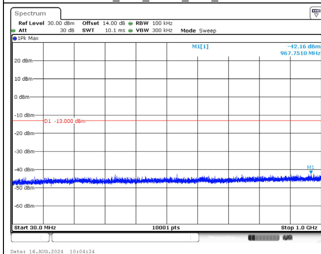
2593.0 MHz_10M_QPSK_1RB_Below 1GHz
