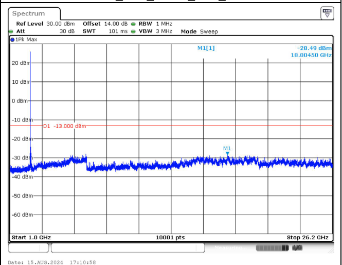
2610.0 MHz _20M_QPSK_1RB_Above 1GHz
