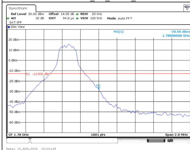
1777.5 MHz _5M_QPSK_1RB
