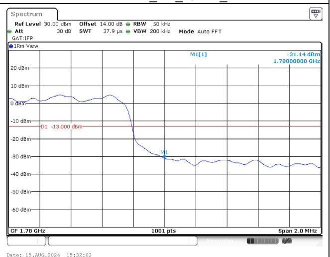
1777.5 MHz _5M_QPSK_FRB
