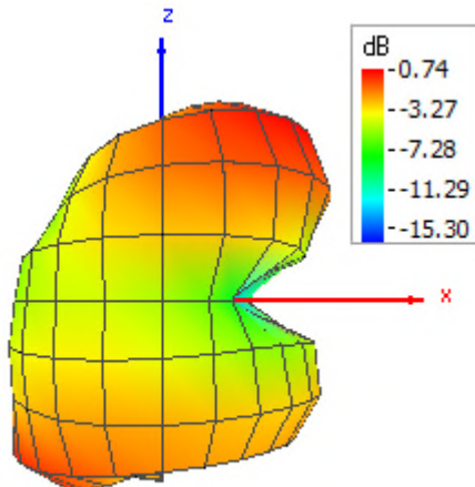
Fig 4: 3D OTA test result: Antenna pattern for 2480 MHz. Test antenna input power setting was 0 dBm.
