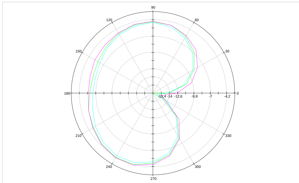
Fig 5: MainCutsPlot_XY_Plane
