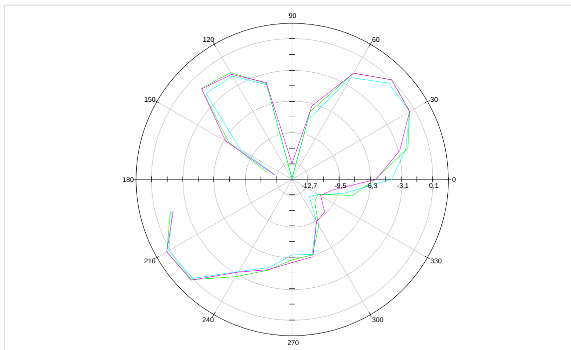
Fig 6: MainCutsPlot_XZ_Plane
