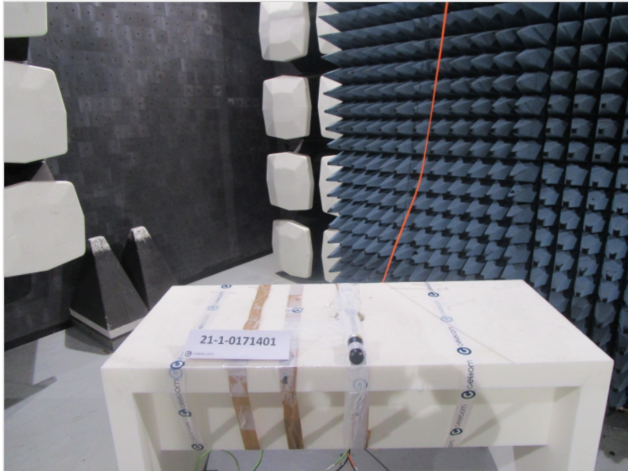
Photograph 1: EUT test setup in the semi anechoic chamber, close up view_EUT elevation 0°
