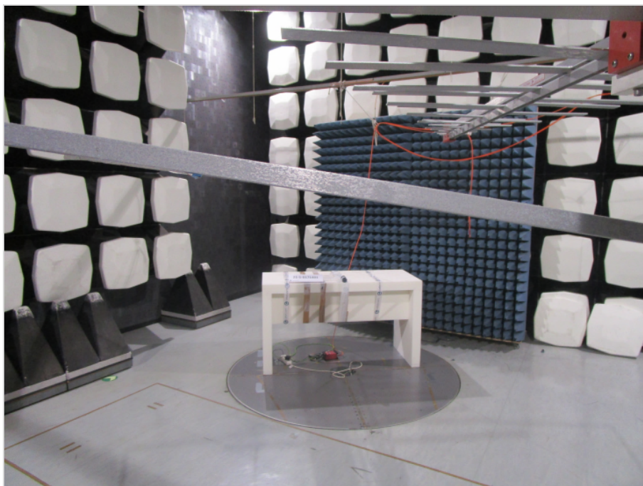
Photograph 2: EUT test setup in the semi anechoic chamber, overview_EUT elevation 0°
