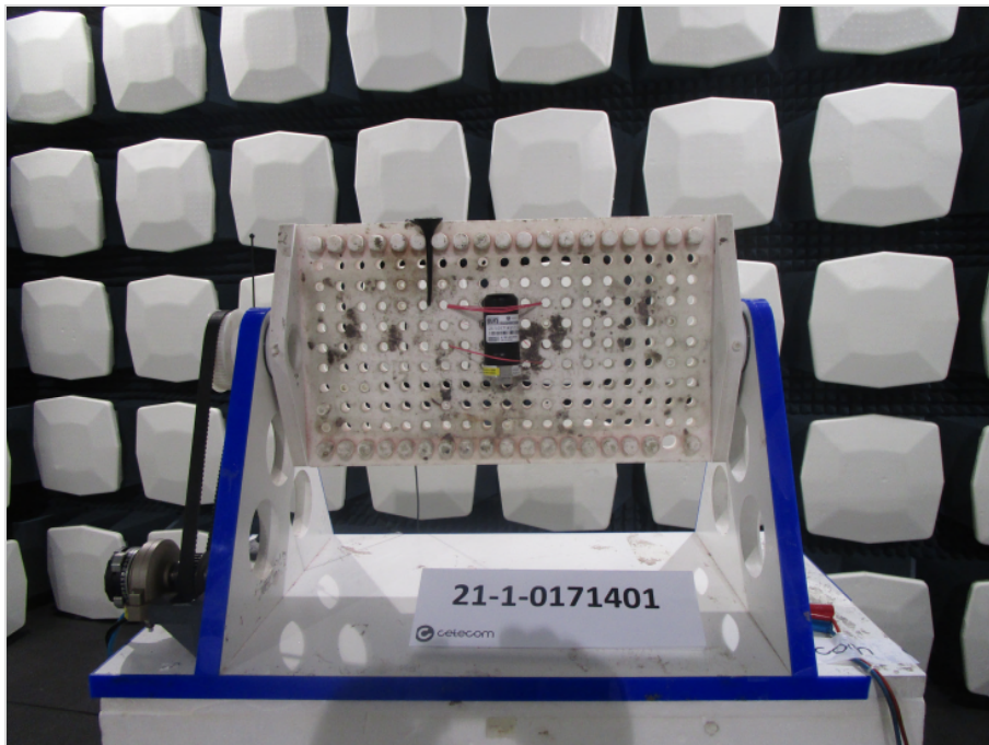
Photograph 5: EUT test setup in the fully anechoic chamber, close up view_EUT
