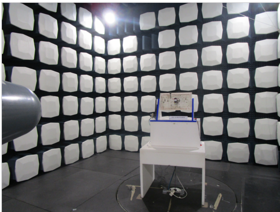
Photograph 6: EUT test setup in the fully anechoic chamber, overview_EUT
