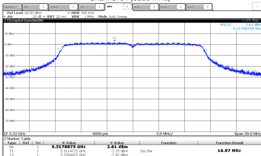
Channel 64 (5320 MHz)
