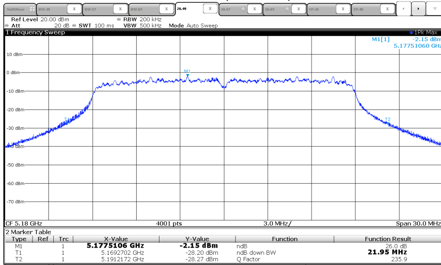
Channel 36 (5180 MHz)
