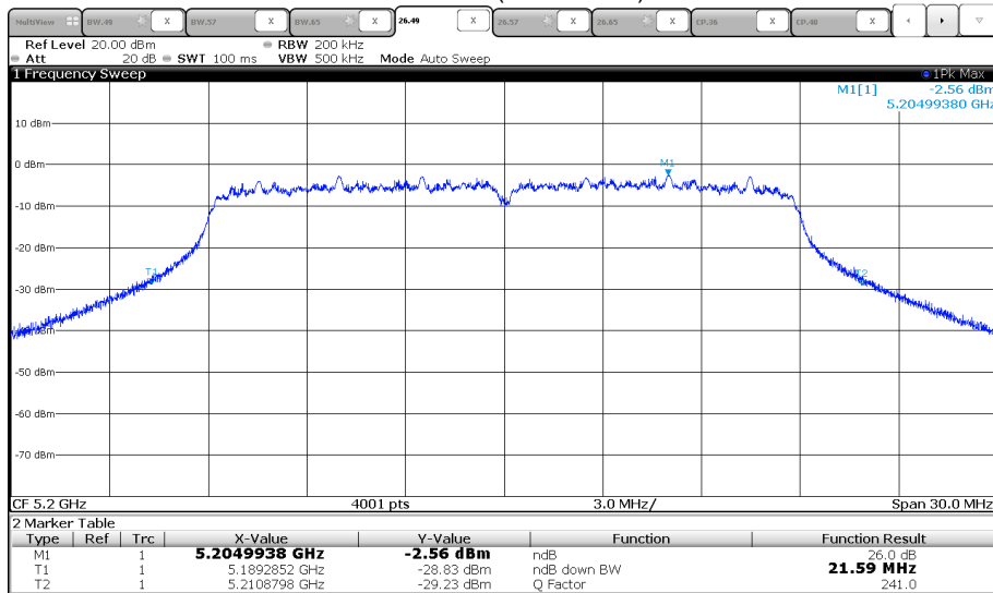
Channel 40 (5200 MHz)
