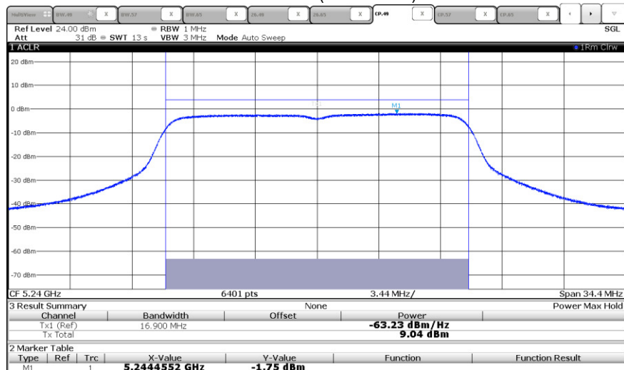
Channel 48 (5240 MHz)
