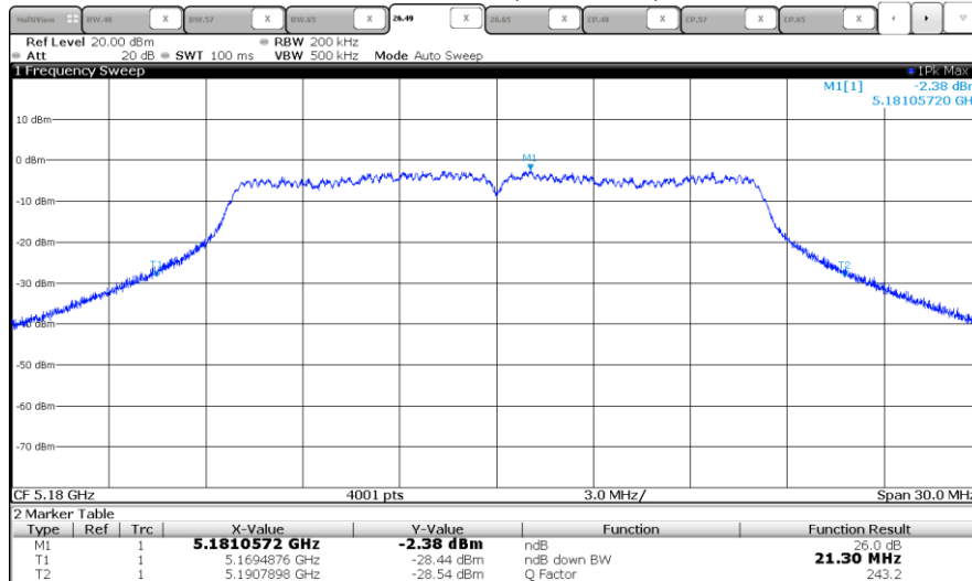
Channel 36 (5180 MHz)
