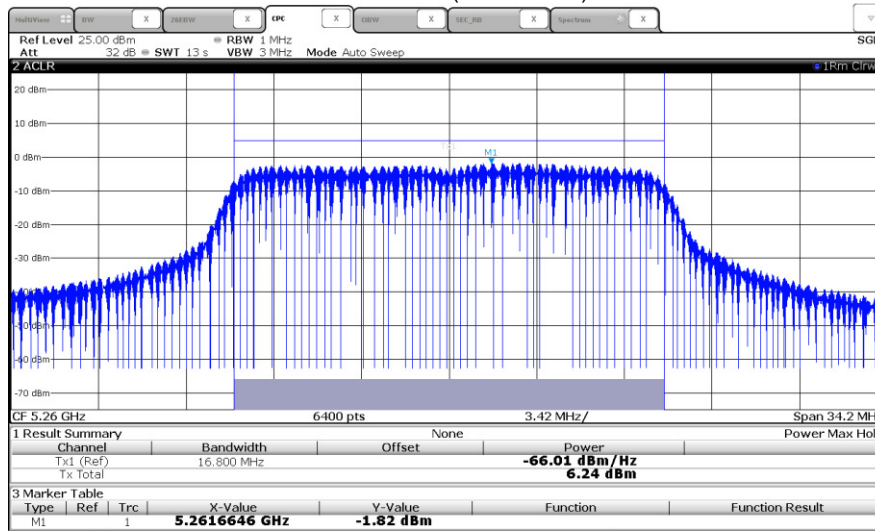
Channel 52 (5260 MHz)
