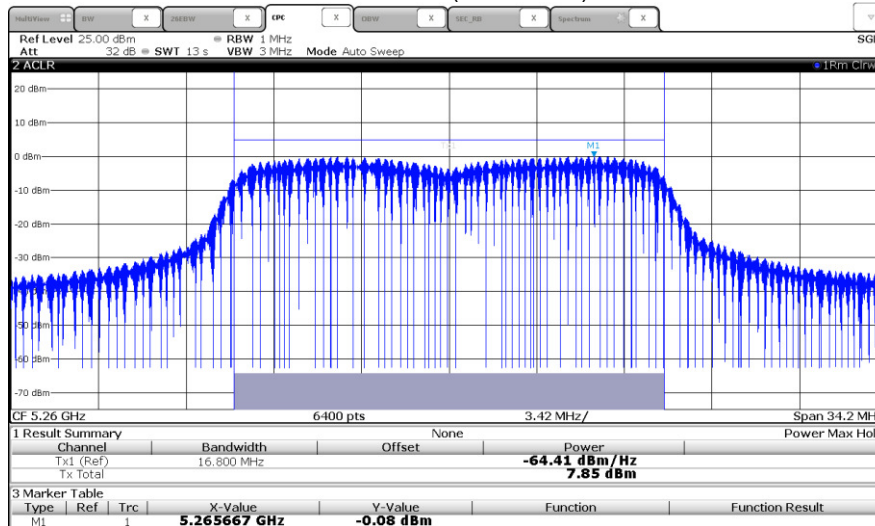
Channel 52 (5260 MHz)
