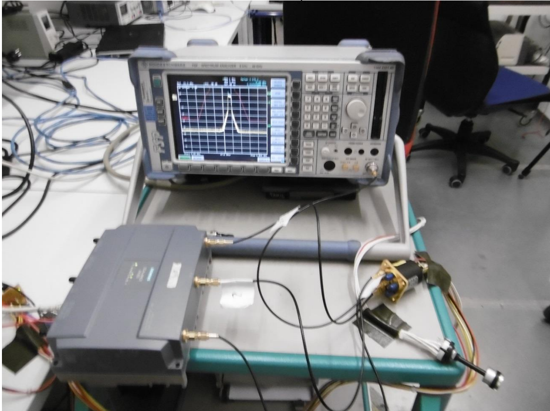
Test setup
