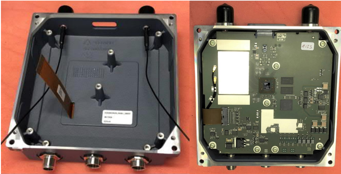
Case Inside – Interface board
