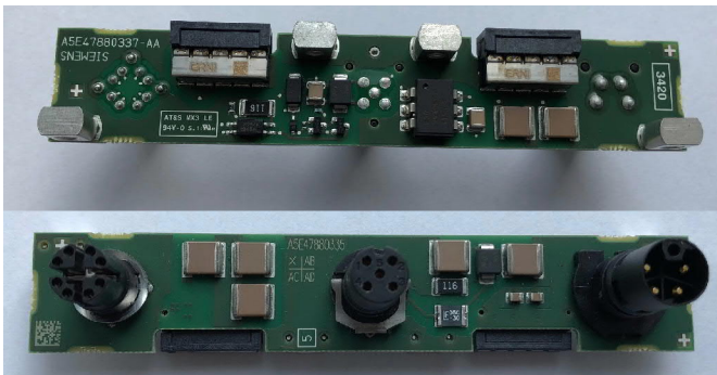
Interface Board A-Side and B-Side
