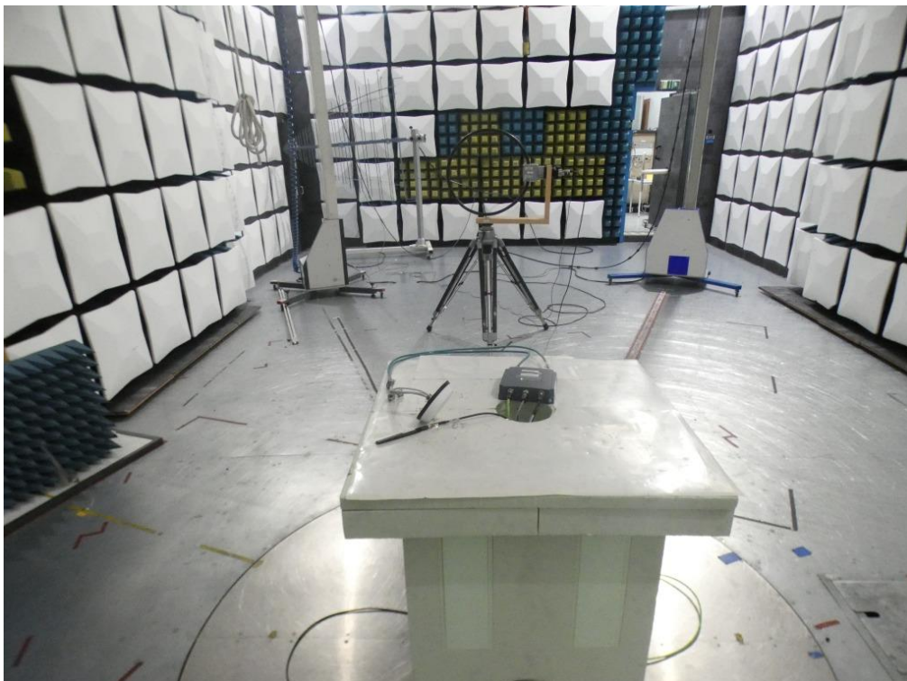
Photo 2/3: Test setup for radiated measurements Semi Anechoic Chamber.
