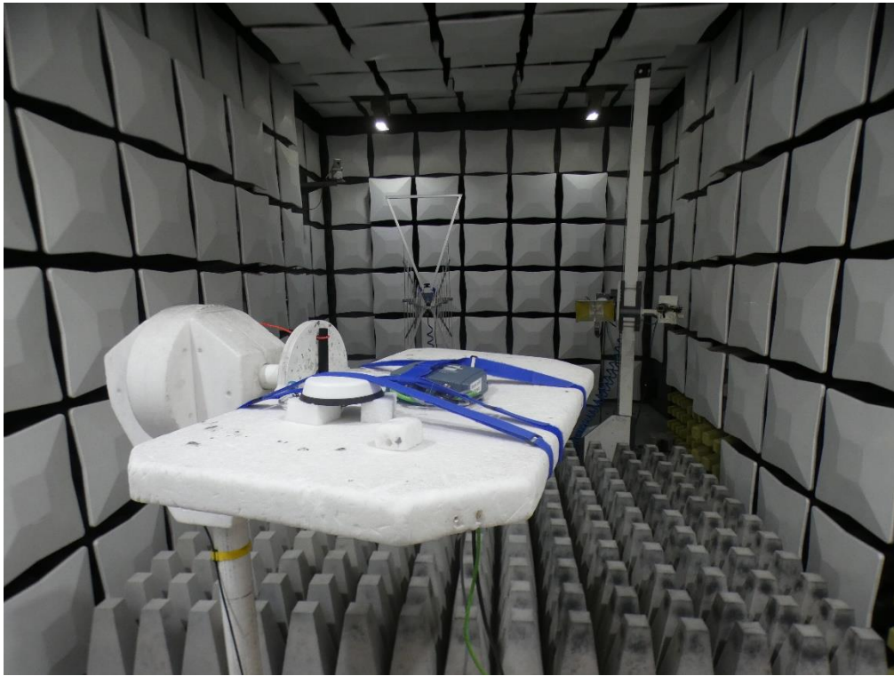
Photo 1: Test setup for radiated measurements Fully Anechoic Chamber.
