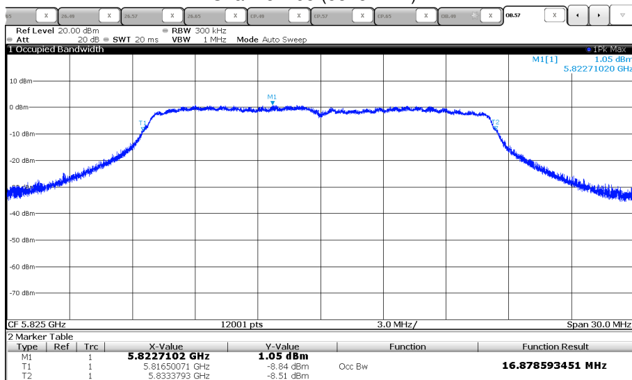
Channel 165 (5825 MHz)
