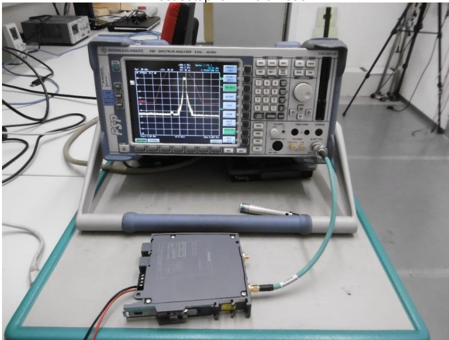
Test setup for 1 Port mode
