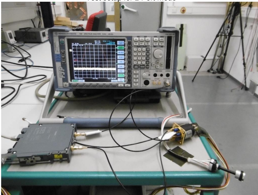
Test setup for 2 Port mode
