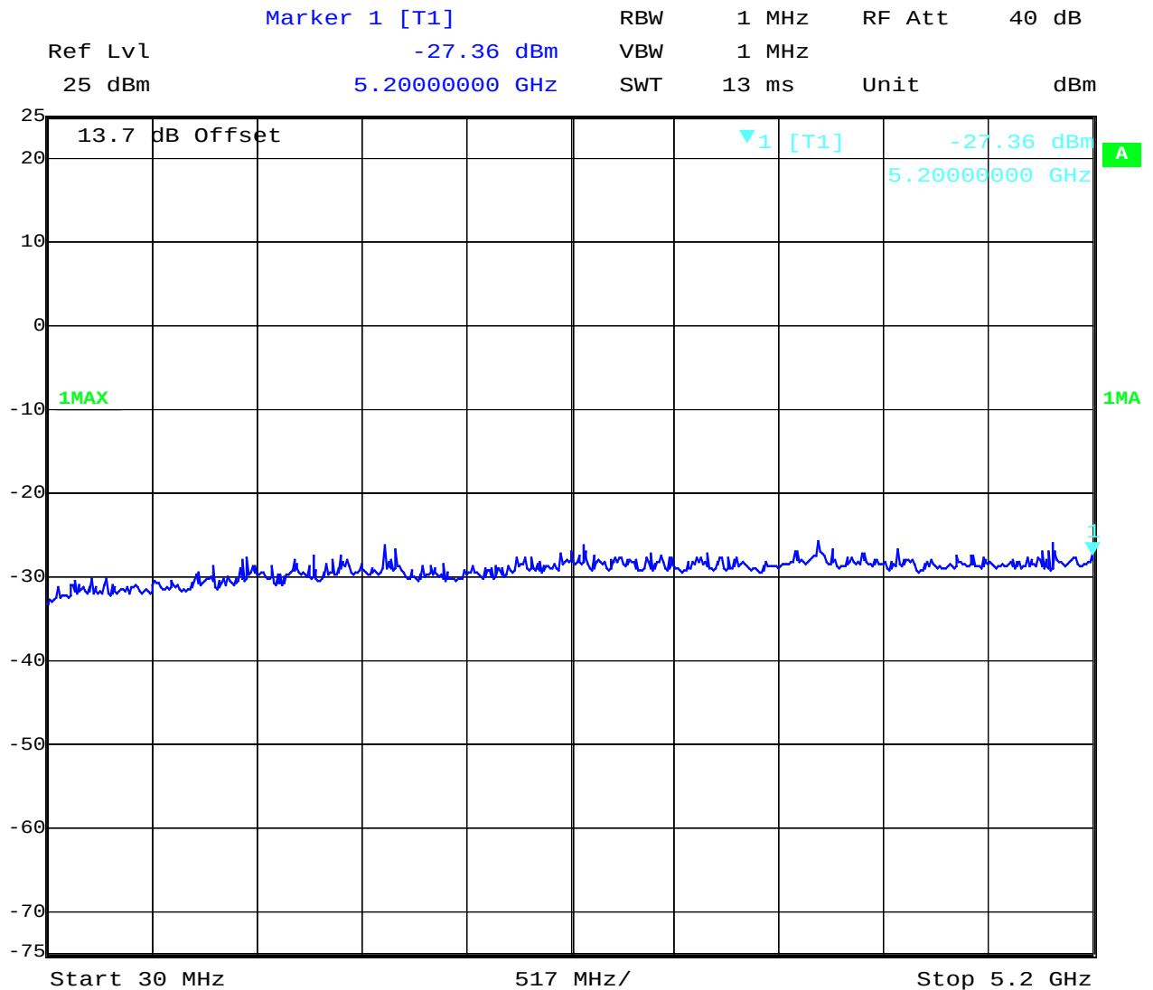
Plot 5: 5300 MHz
