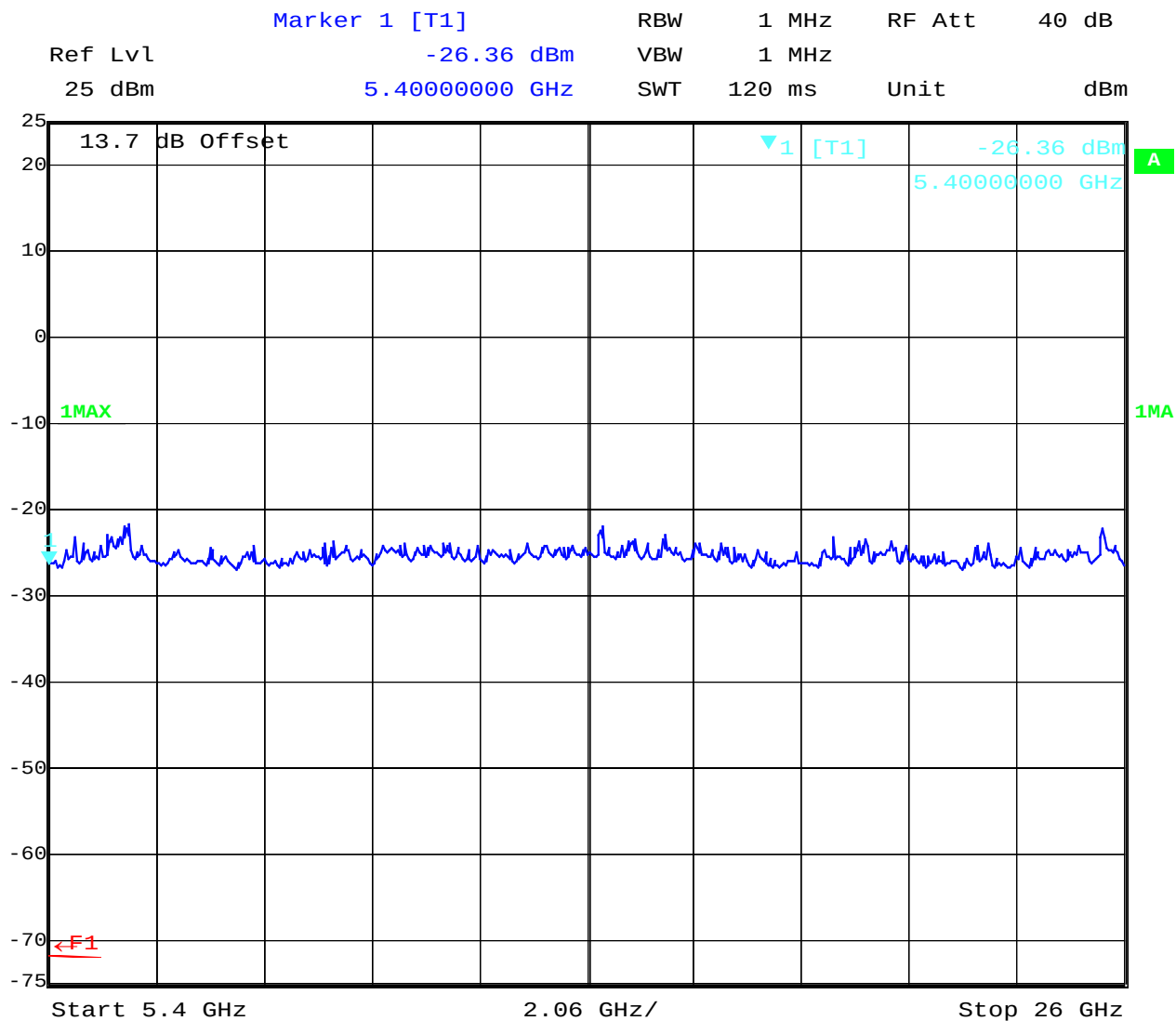
Plot 8: 5320 MHz
