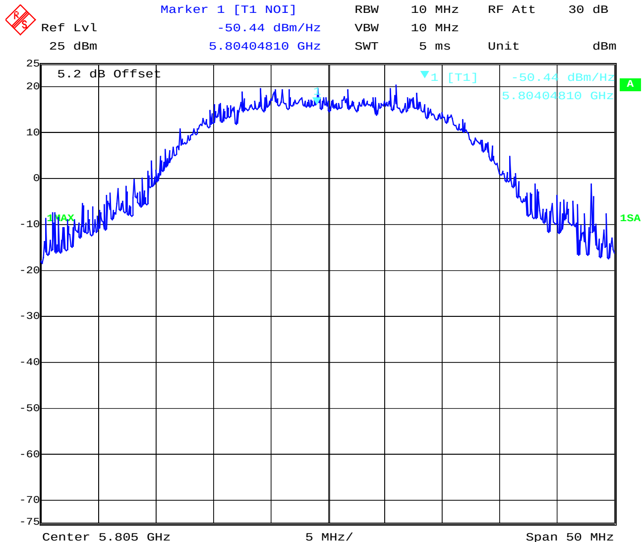
Plot 4: 5805 MHz
