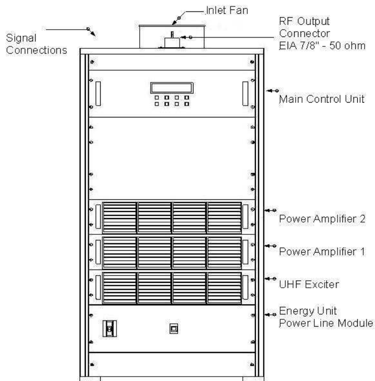
Fig1.1: AT7400 Front View, cabinet wheels are optional.
