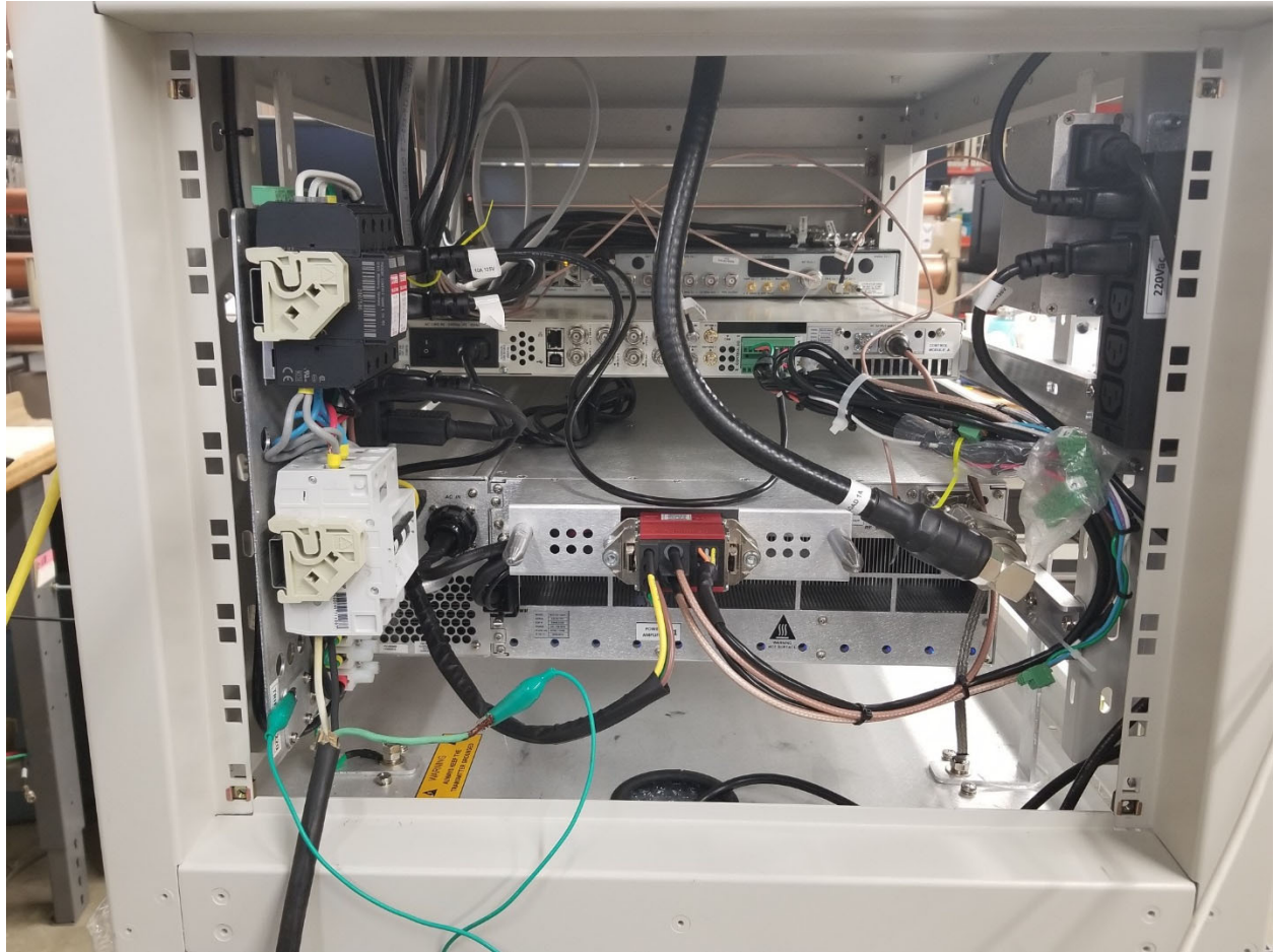
Figure 2. EC-701HP Rear View
