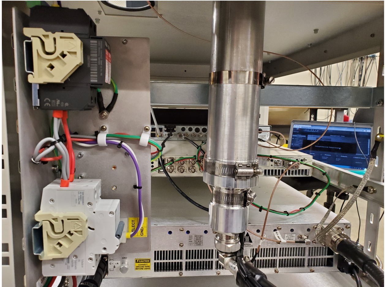
Figure 2. EC706HP-BB2 Rear View
