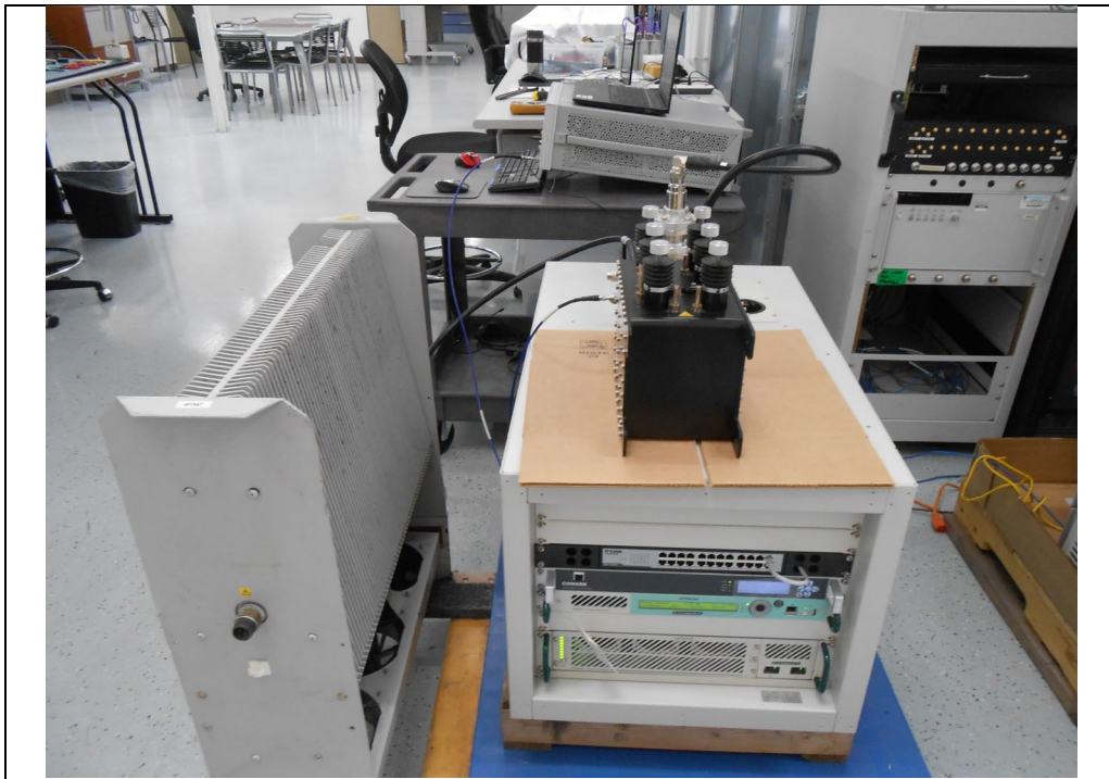
RF Conducted #1
