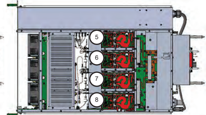
POWER AMPLIFIER DRAWER Bottom View
