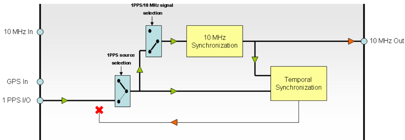
Figure 15: VX20-x0x2 clock synchronization – external 1PPS signal
