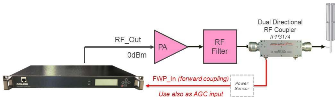
Figure 20: Built-in output AGC
