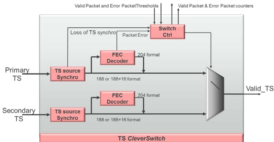
Figure 2: TS CleverSwitch block diagram
