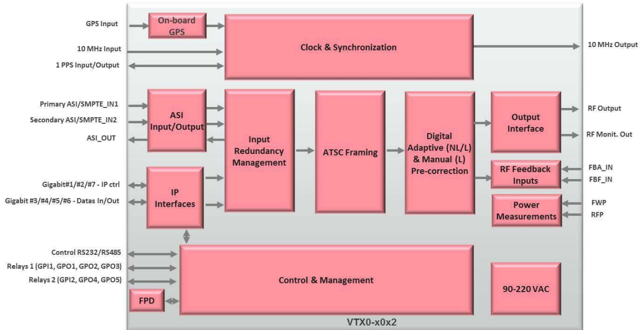
Figure 1: EXACT-V2 functional block diagram
