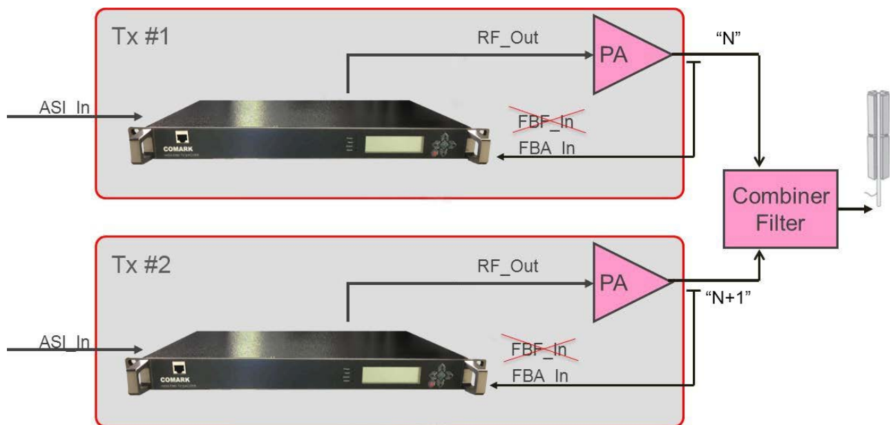
Figure 5: Manual Linear Precorrection use-case – Combined filter
