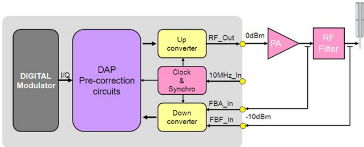
Figure 6: DAP integration block diagram
