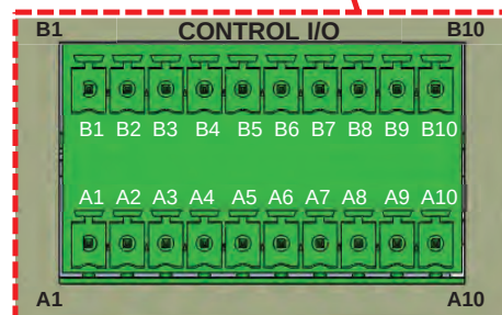
Control I/O connector Rear panel
