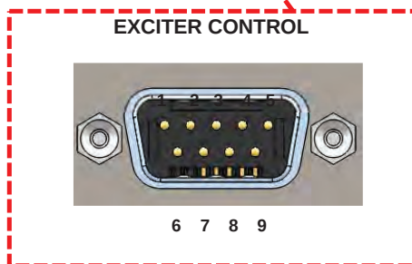
DB9 male connector Rear panel
