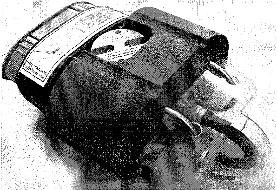
ADT 406 S General view with its bracket mount, protective cover and whip antenna
