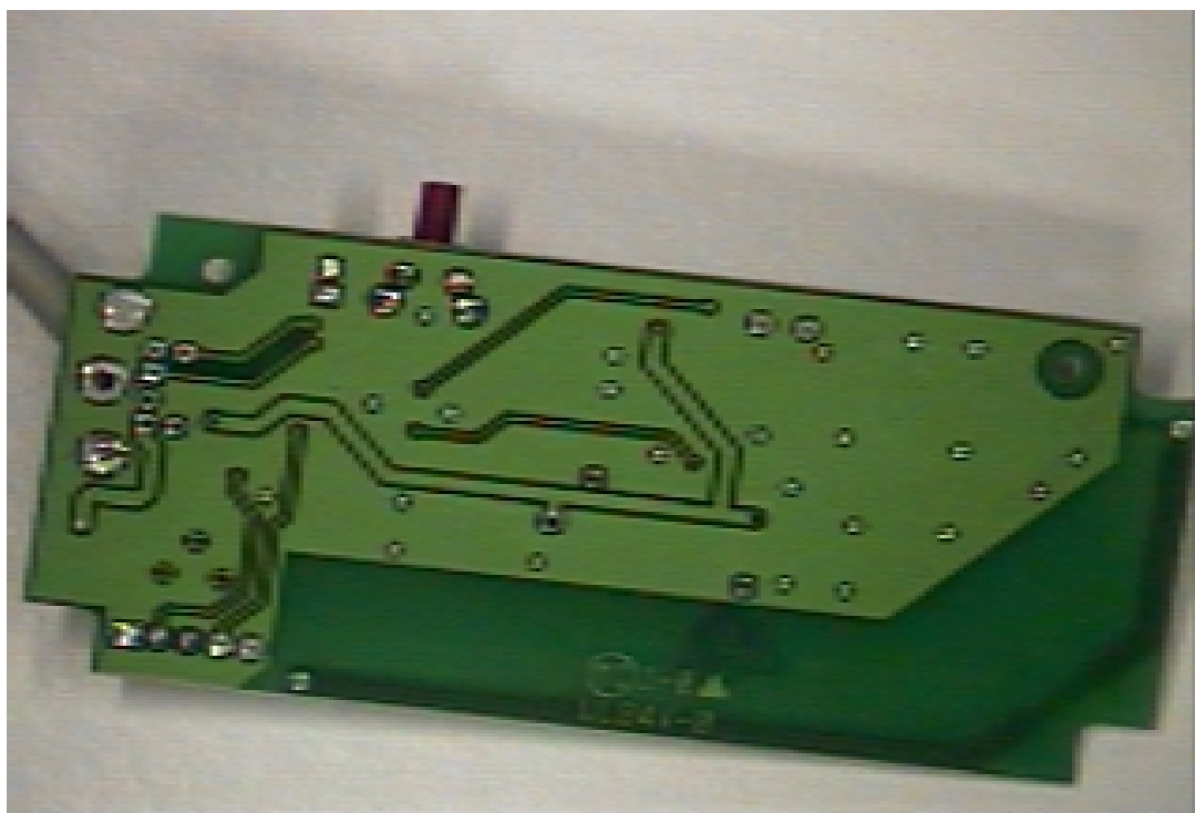
Foil side of Receiver PCB
