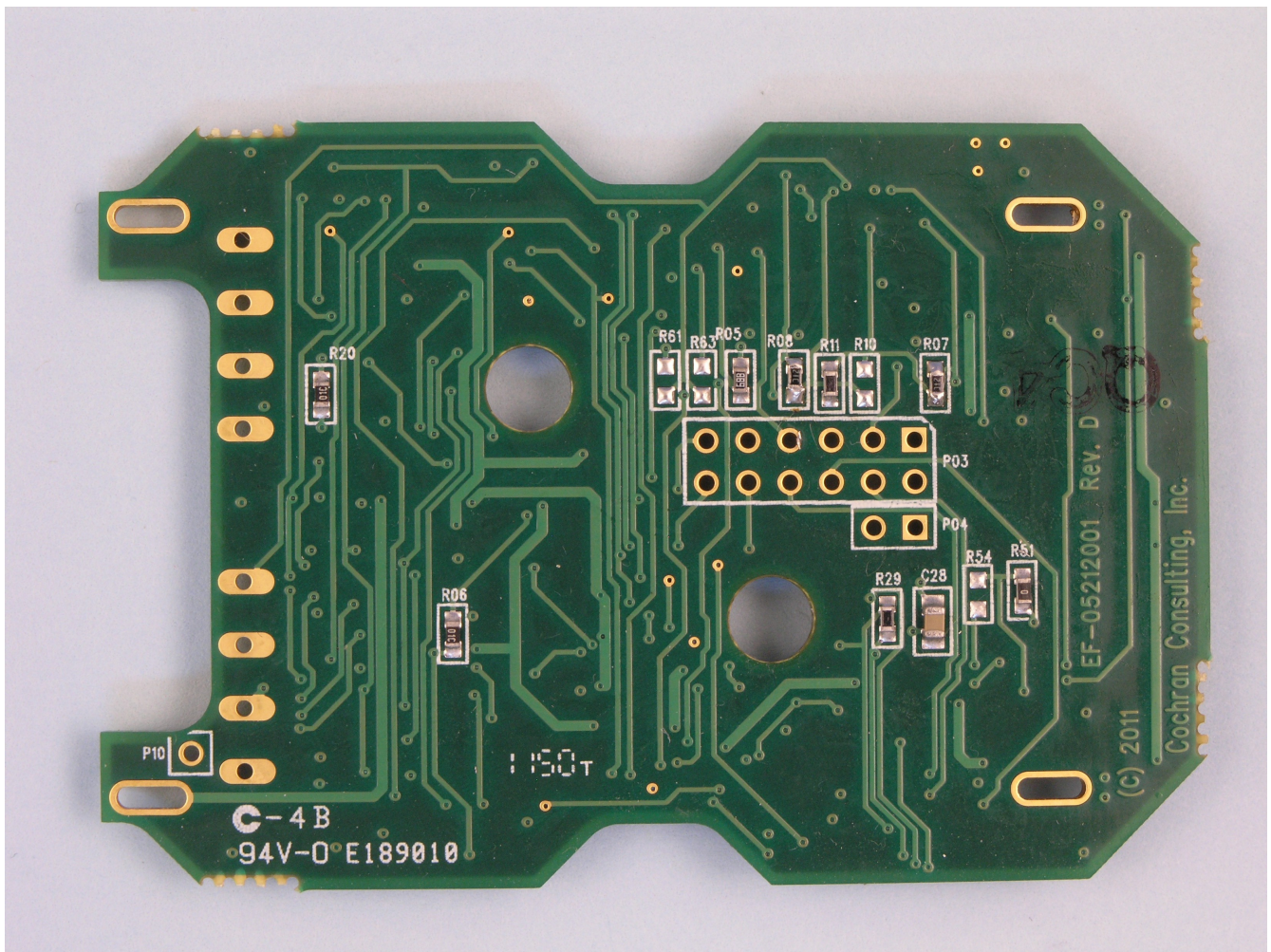
Lifeguard FCC ID: LYP44556-05 Analog PCB Back/Bottom View
