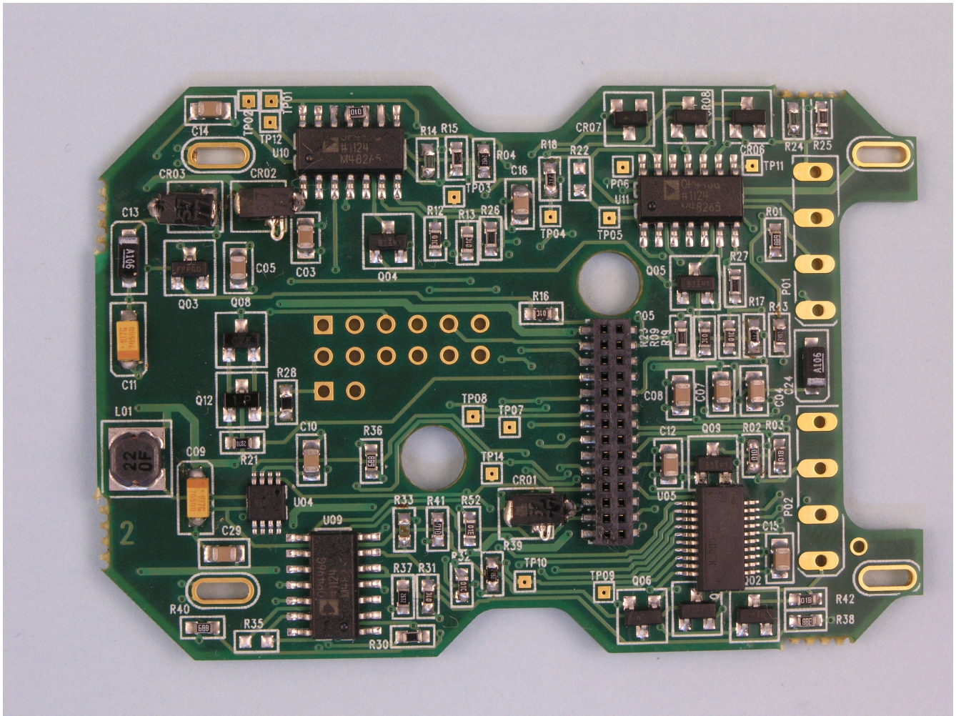
Lifeguard FCC ID: LYP44556-05 Analog PCB Front/Top View
