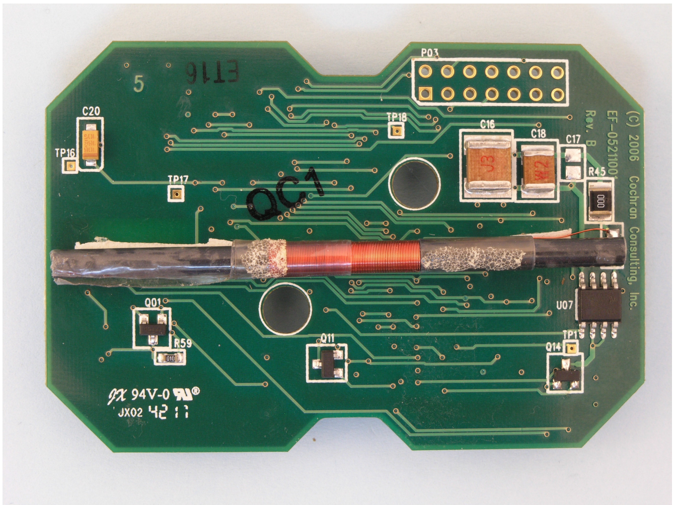
Lifeguard FCC ID: LYP44556-05, PCB Front/Top View
