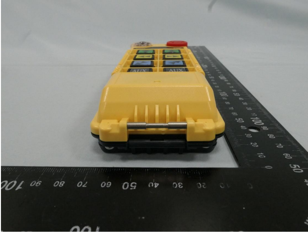
(4) EUT Photo - Alpha 608XJ (Remote Control TX)
