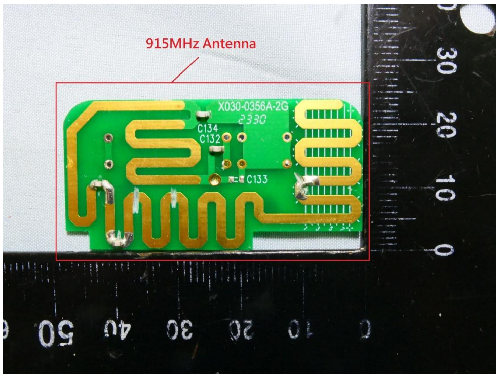
(10) EUT Photo - Alpha 608XJ (Remote Control TX)
