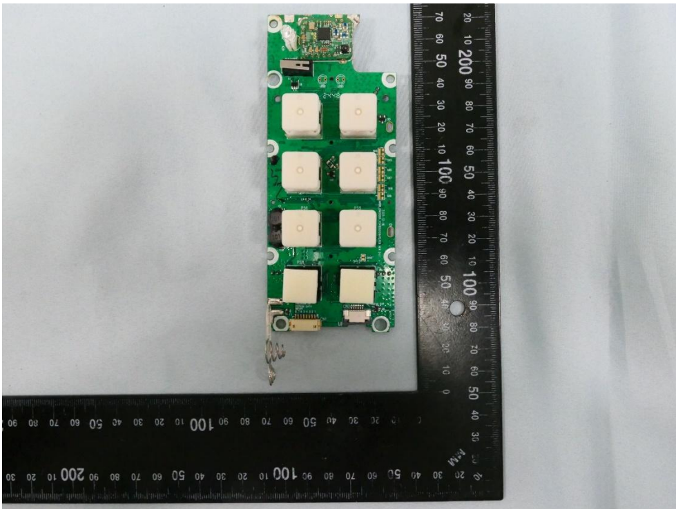
(6) EUT Photo - Alpha 608XJ (Remote Control TX)
