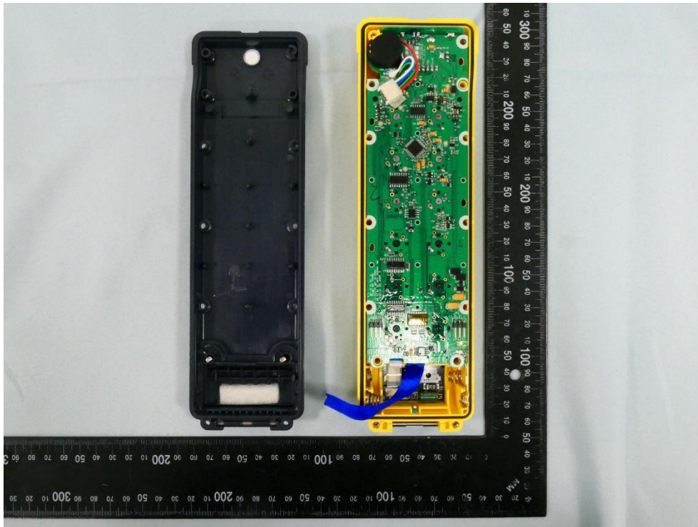
(2) EUT Photo - Alpha 612XJ (Remote Control TX)
