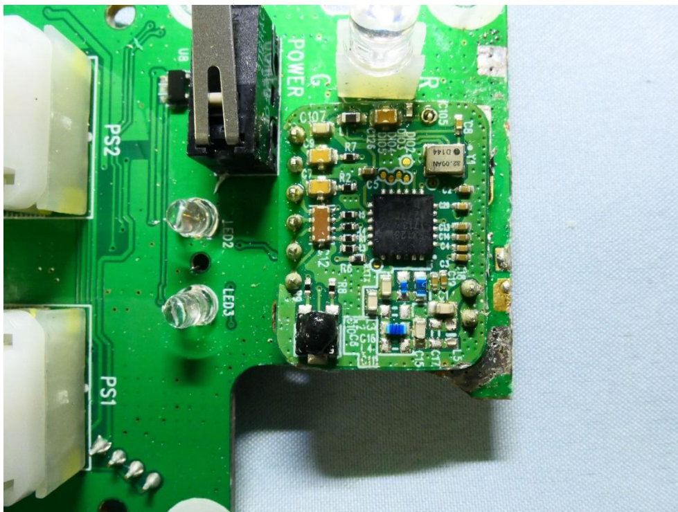
(8) EUT Photo - Alpha 612XJ (Remote Control TX)
