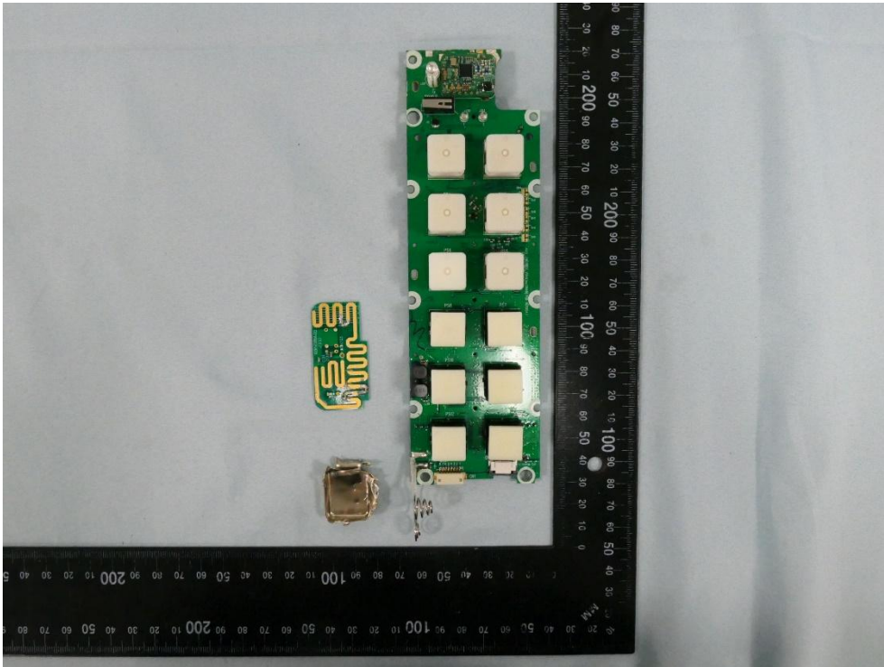
(6) EUT Photo - Alpha 612XJ (Remote Control TX)
