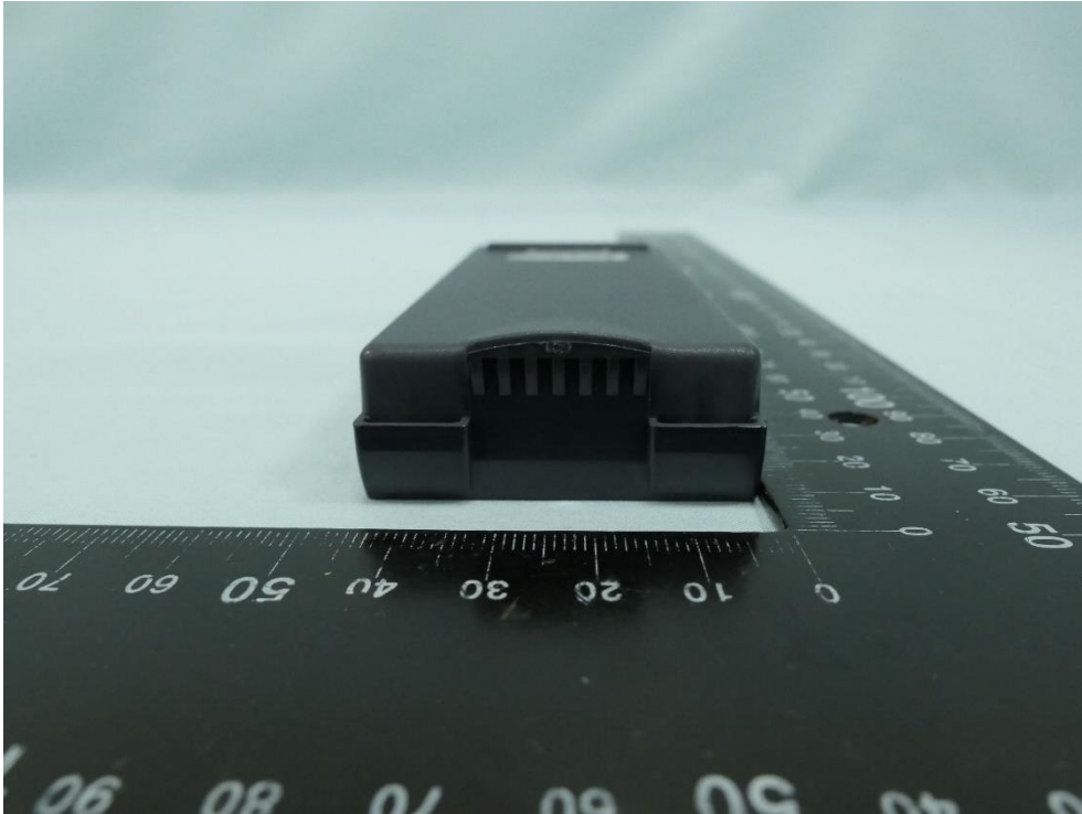
(10) Battery Photo
